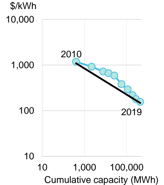
Batteries pack price ($/kWh)
