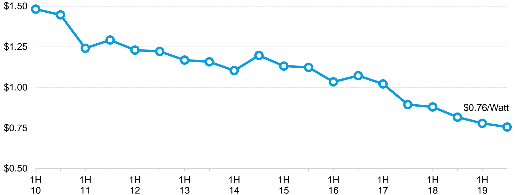
Wind turbine price index by turbine delivery date
