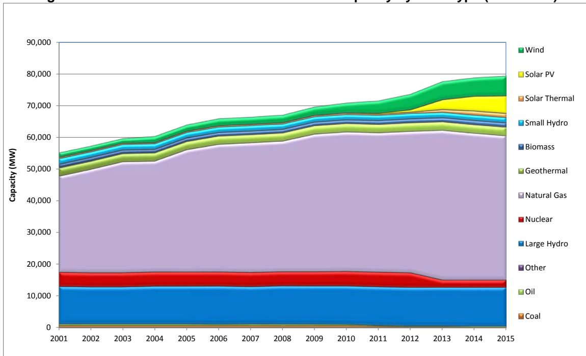
Figure 1: Installed In-State Electric Generation Capacity by Fuel Type (2001-2015)
