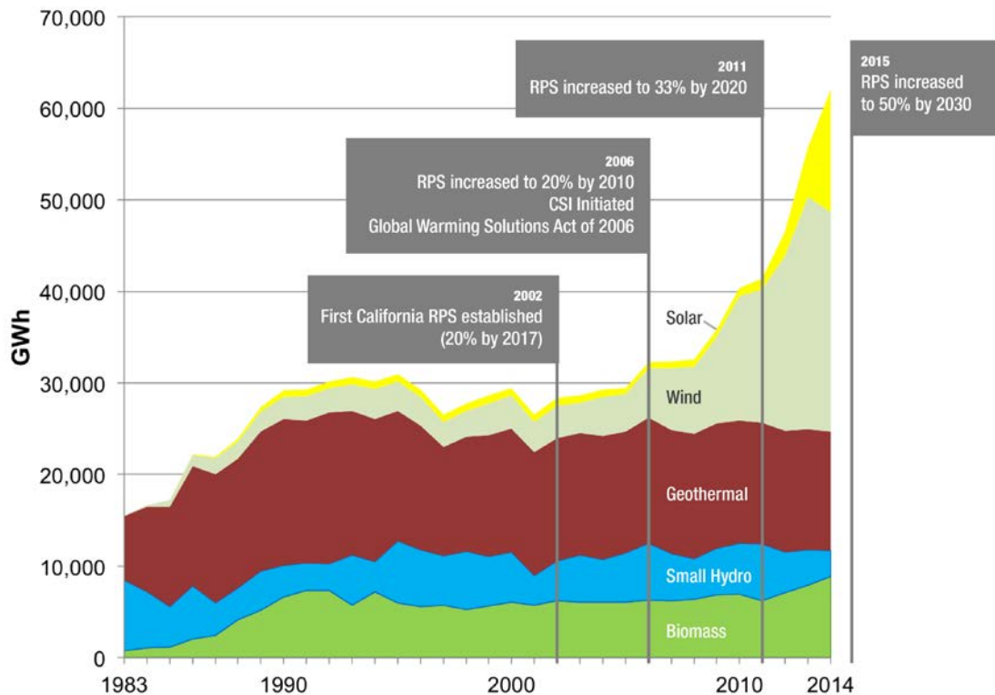
Figure 3: California Renewable Energy Generation From 1983-2014 by Resource Type (In-State and Out-of-State)
