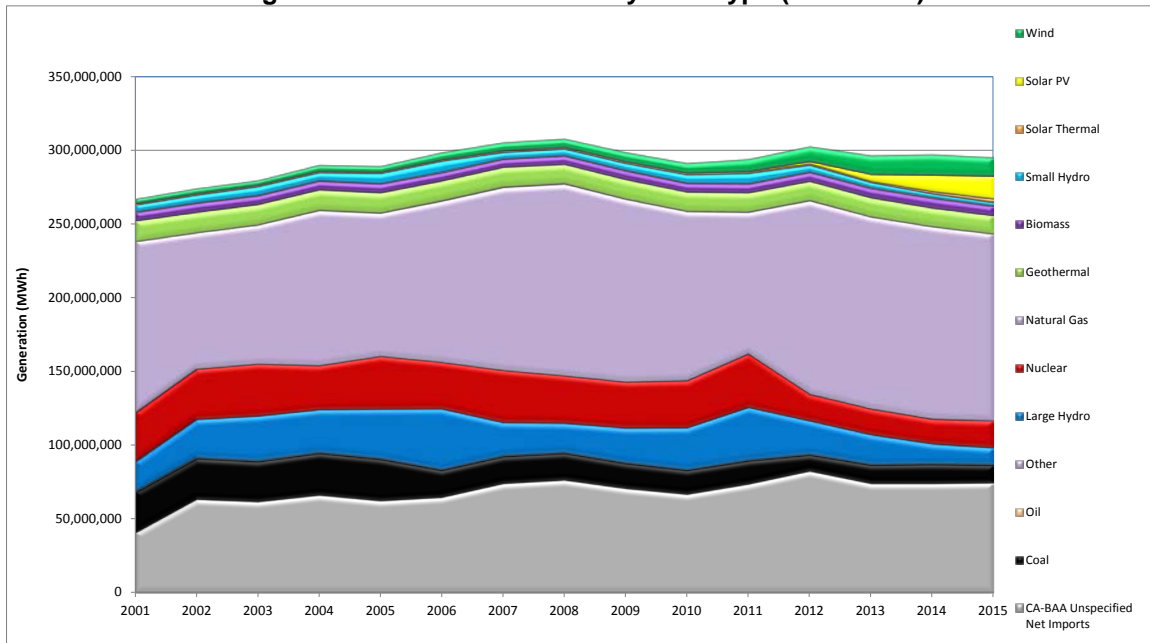
Figure 2: Electric Generation by Fuel Type (2001-2015)
