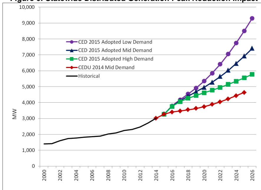
Figure 6: Statewide Distributed Generation Peak Reduction Impact
