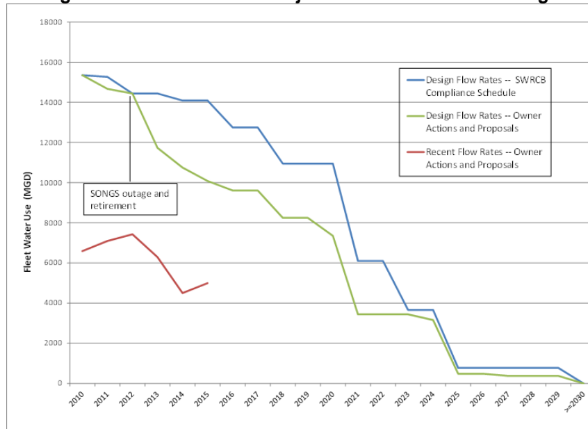
Figure 23: Historical and Projected OTC Fleet Water Usage
