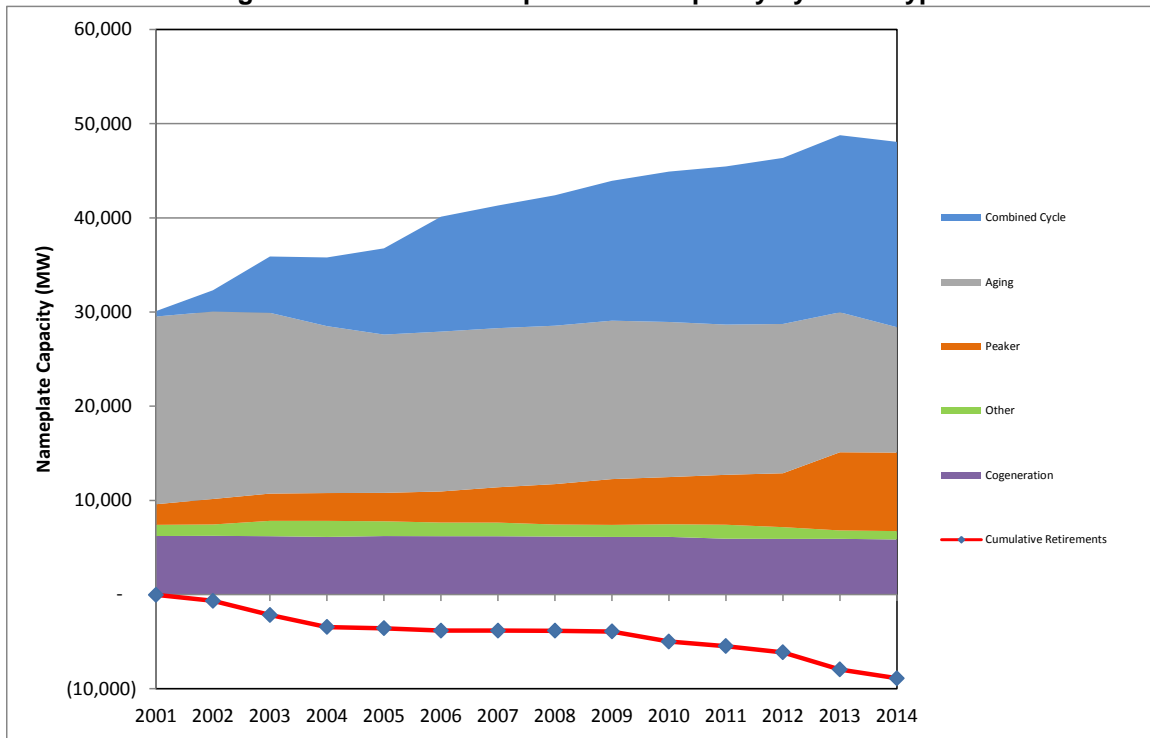
Figure 8: Total Annual Operational Capacity by Plant Type
