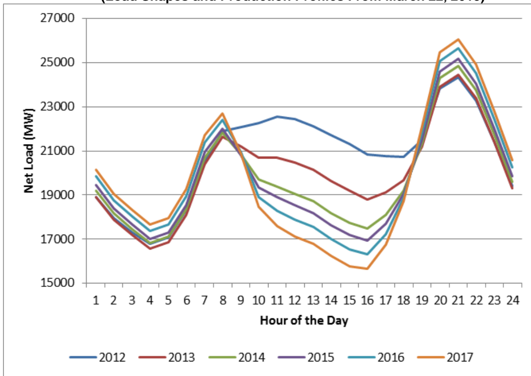
Figure 9: Illustrative Change in Net Load Curves (Load Shapes and Production Profiles From March 22, 2013)
