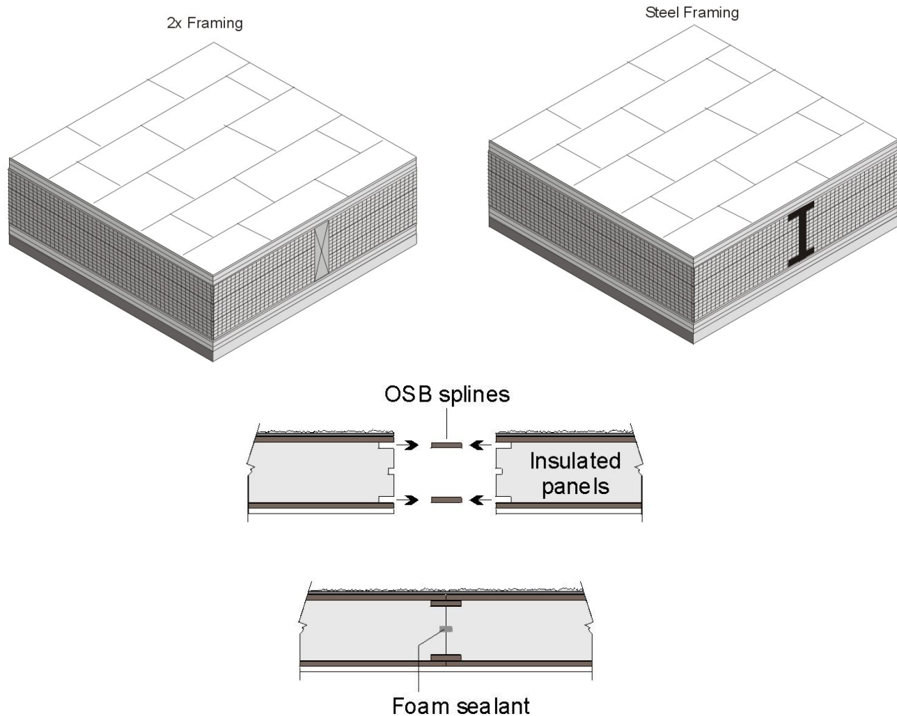
Figure 4.2.4 – SIPs Roof/Ceiling
