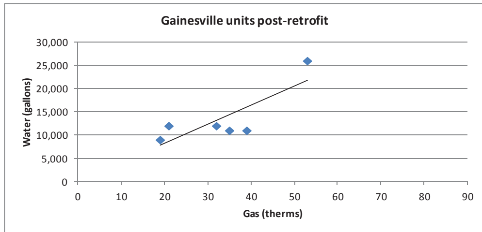
Figure G.2. Plot of water and gas use in the post-retrofit study period in the Gainesville units
