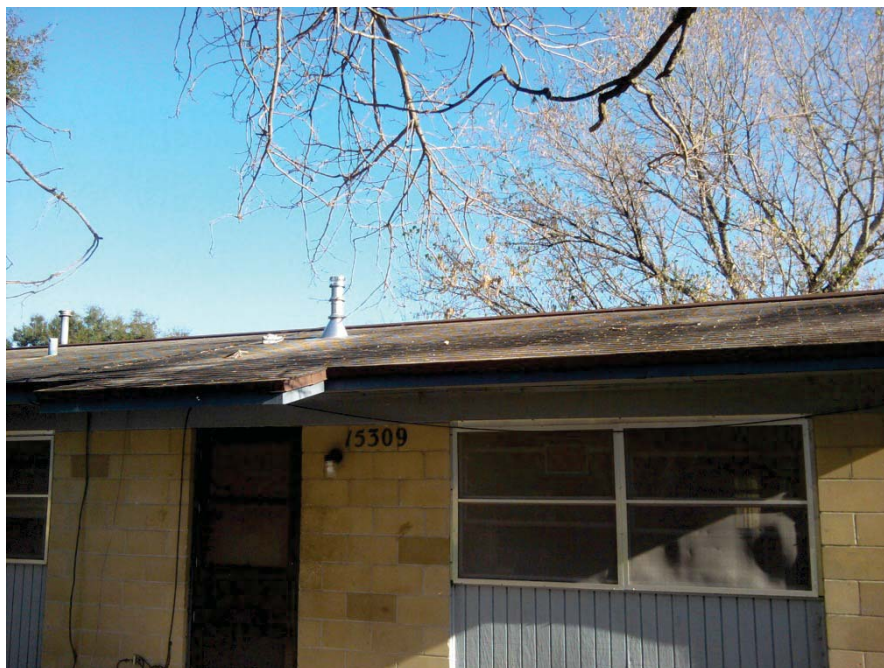
Figure L.2. Actual vertical venting assembly attached to the roof
