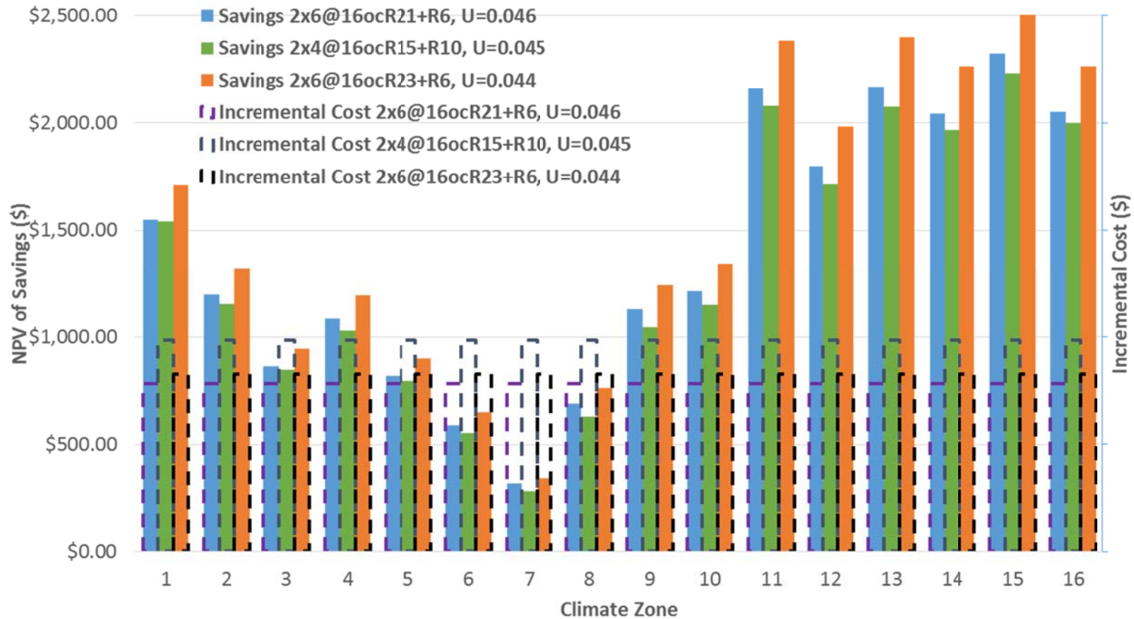
Figure 3: Energy Savings and Incremental Costs of Assemblies with U-factors 0.046 or less
