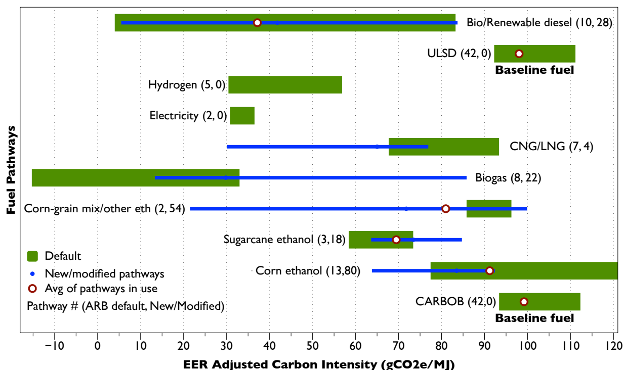
Figure 5. Carbon intensity (CI) ratings of feedstock/fuel combinations in California's LCFS as of April 2014. Green bars represent ARB-derived ratings (pathway defaults). Blue bars represent pathways submitted by regulated parties (through Methods 2A and 2B). Red circles represent the average CI ratings of individual biofuel pathways in use (both defaults and new/modified (not weighted by volume)). California Reformulated Gasoline Blendstock for Oxygenate Blending (CARBOB) and Ultra-Low Sulfur Diesel (ULSD) pathway values are calculated using country of crude oil origin; the mean is the reference fuel value used in the regulation. Modified values can be higher than the defaults for a particular feedstock/fuel combination due to differences in technologies used. CI values are adjusted with an energy efficiency ratio (EER) of 3.4 for electricity. "Corn-grain mix/other" ethanol pathways include corn/sorghum, corn/sorghum/wheat mixes, and ethanol from sorghum, molasses, and waste beverages.
