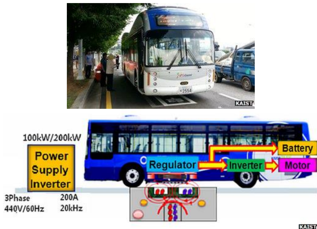
Figure 3.7 The Korean Advanced Institute of Science and Technology (KAIST) Buses a
