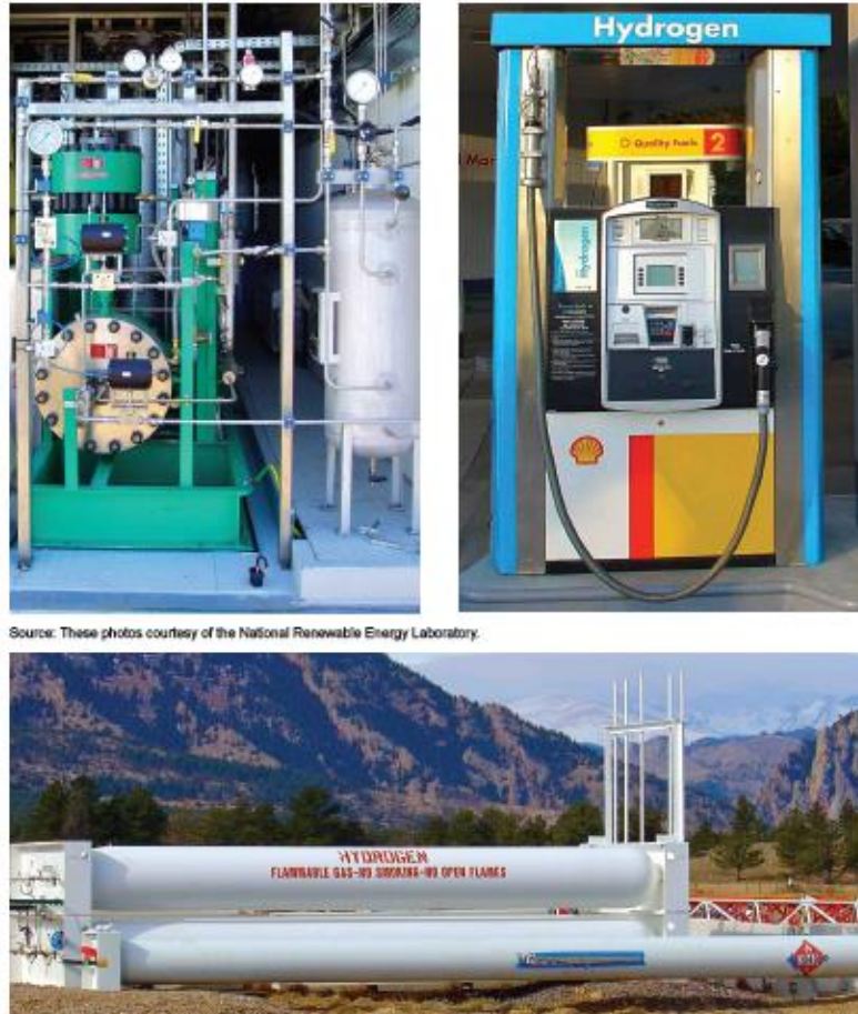
Figure 3.5 Typical Onsite Compression, Dispensing, and Storage Equipment for H 2
