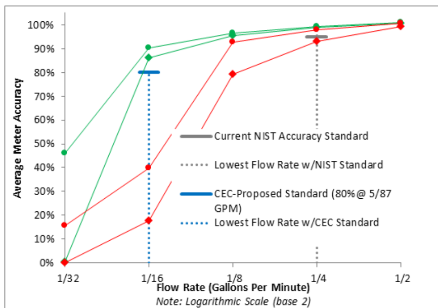
Figure C.1 Average Performance of 5/8 x 3/4" Positive Displacement (Piston and Disc) Meters
