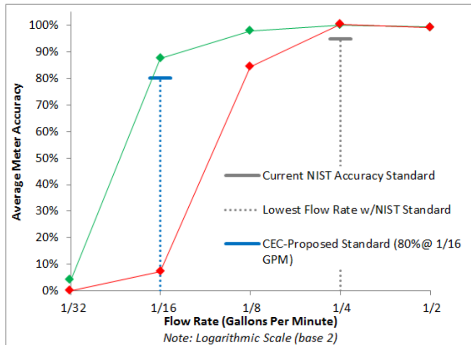
Figure C.3 Average Performance of 5/8 x 3/4" Single Jet Meters
