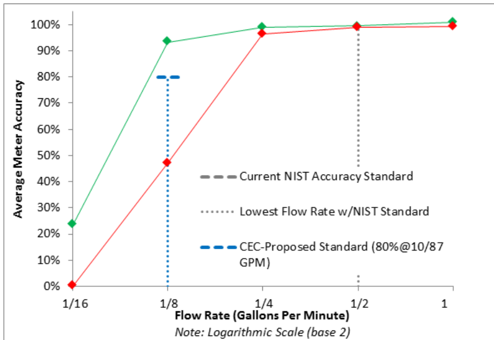
Figure C.6 Average Performance of Qualifying and Non-qualifying 3/4" Single Jet Meters
