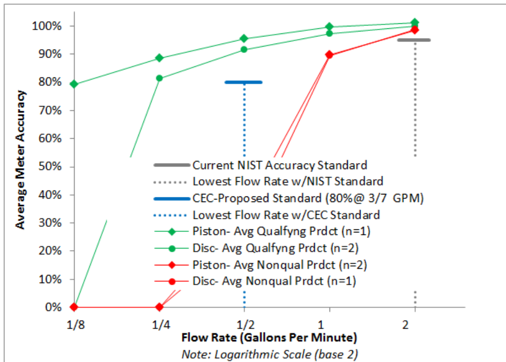
Figure C.12 Average Performance of 2" Positive Displacement (Piston and Disc) Meters
