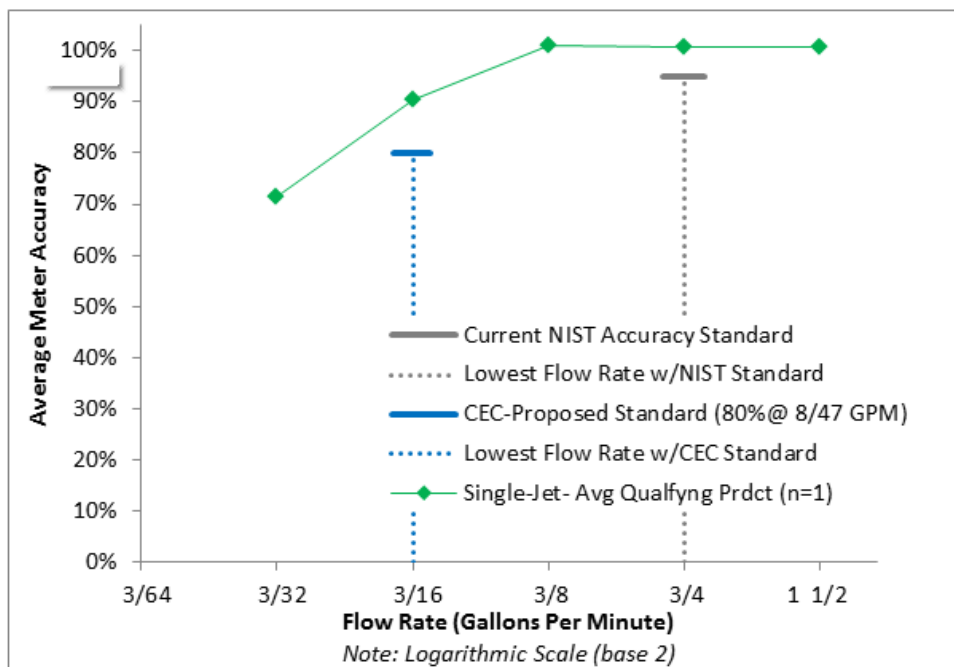
Figure C.11 Average Performance of 1 1/2" Single Jet Meters
