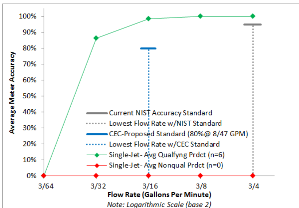
Figure C.9 Average Performance of Qualifying and Non-qualifying 1" Single Jet Meters
