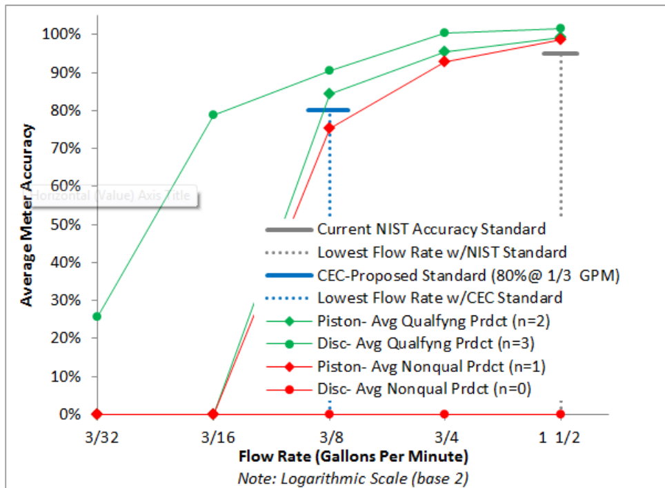
Figure C.10 Average Performance of 1 1/2" Positive Displacement (Piston and Disc) Meters
