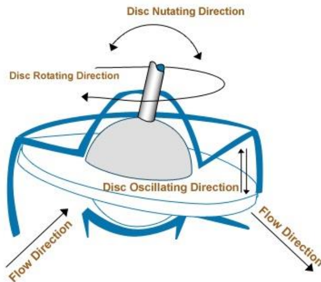
Figure 2.2 Schematic diagram of nutating disc meter measuring chamber
