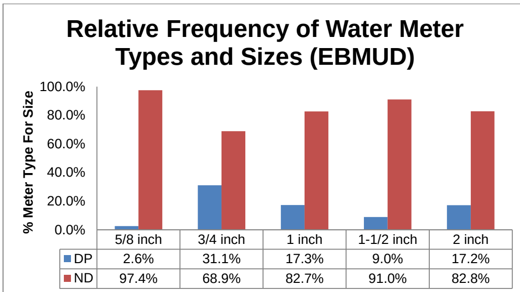
Figure B.2 Distribution of Water Meter Types
