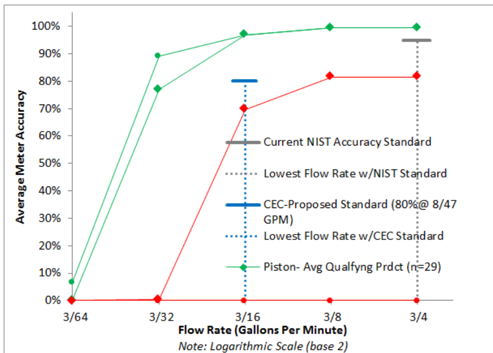
Figure C.7 Average Performance of 1" Positive Displacement (Piston and Disc) Meters
