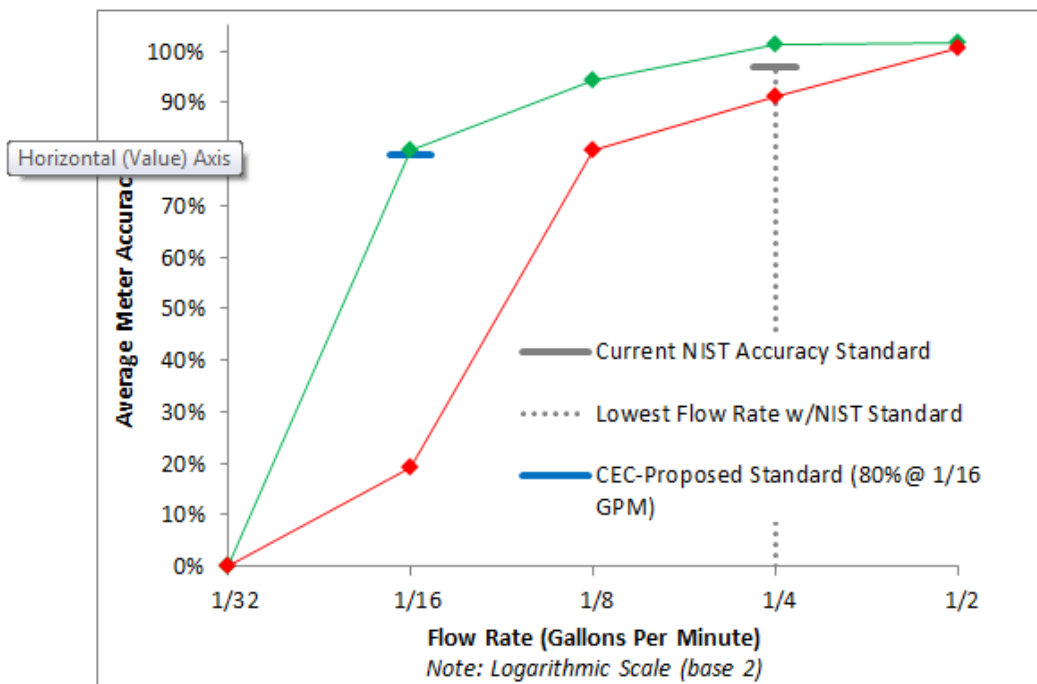
Figure C.2 Average Performance of 5/8 x 3/4" Multi-jet Meters
