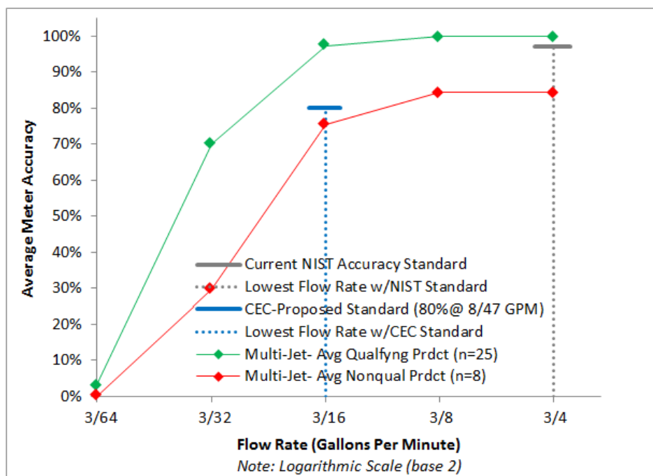
Figure C.8 Average Performance of Qualifying and Non-qualifying 1" Multi-Jet Meters
