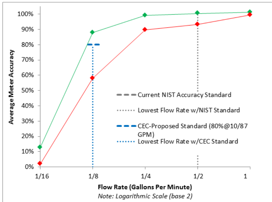
Figure C.5 Average Performance of Qualifying and Non-qualifying 3/4" Multi-Jet Meters
