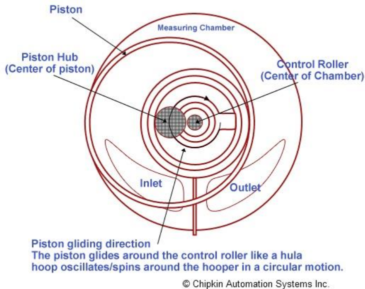
Figure 2.3 Schematic diagram of oscillating piston meter measuring chamber
