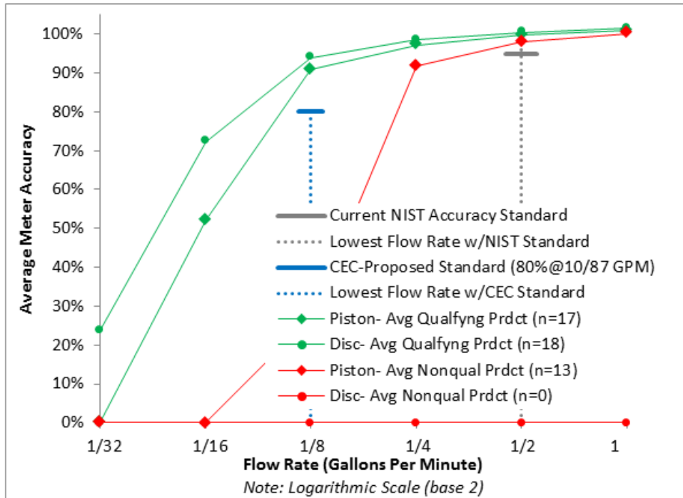
Figure C.4 Average Performance of 3/4" Positive Displacement (Piston and Disc) Meters
