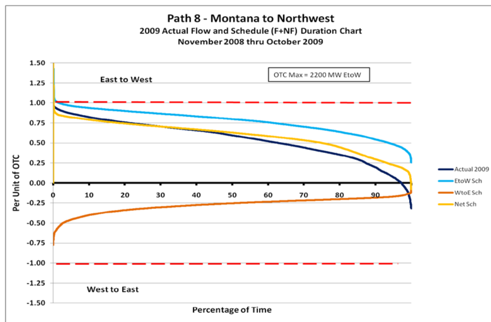
Figure 20: Path 8 Historical Schedule Data Duration Chart
