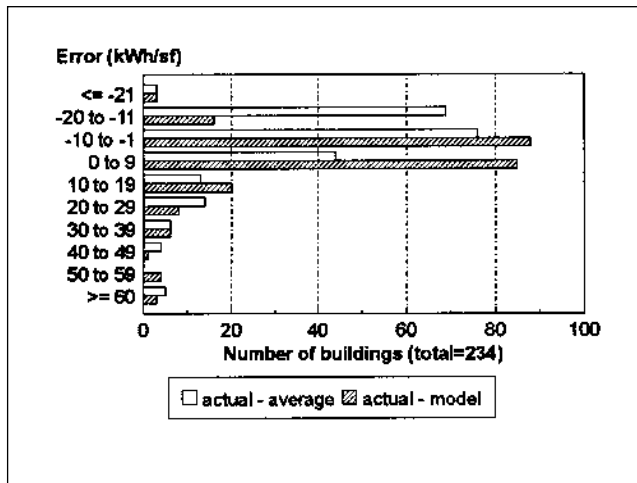
Figure 9. Chart Showing Differences Between Reported and Average EUIs Compared to Differences Between Reported and Model-Predicted EUIs for Census Division 5
