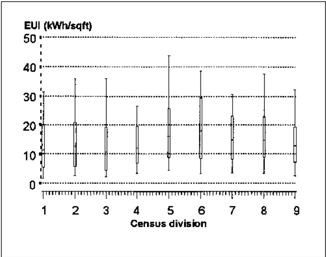
Figure 4. Box Plot Showing Median (Horizontal Line Within Box), 25 and 75% Range Limits (Outer Ends of Box), and 10 and 90% Range Limits (Ends of Stems) for CBECS Office Buildings (Buildings ≤ 1,000,000 sq ft, n = 1358)
