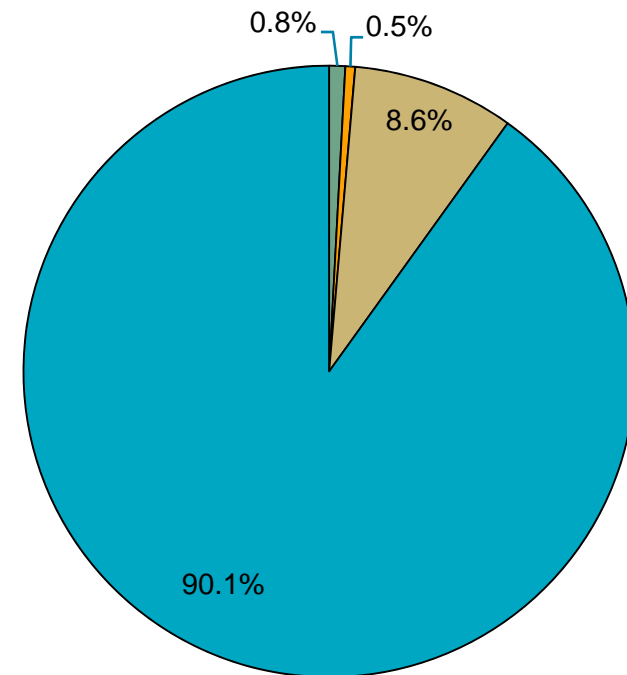
Statewide Emissions 2008 – Particulate Matter
