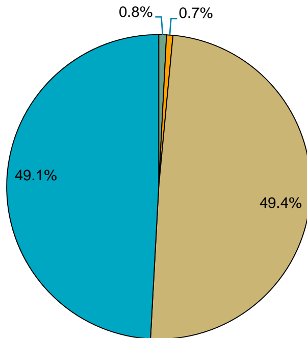
Statewide Emissions 2008 – NO x
