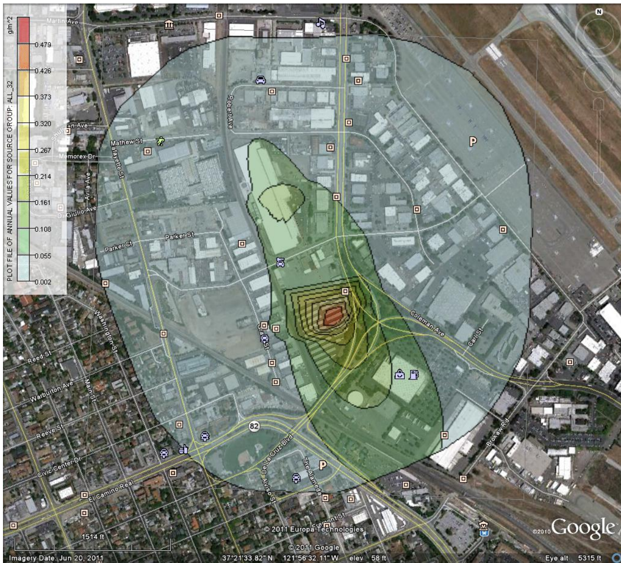
Biological Resources Figure 1. Google map with overlay of modeled nitrogen deposition (g/m 2 ) contour plot (near field view)
