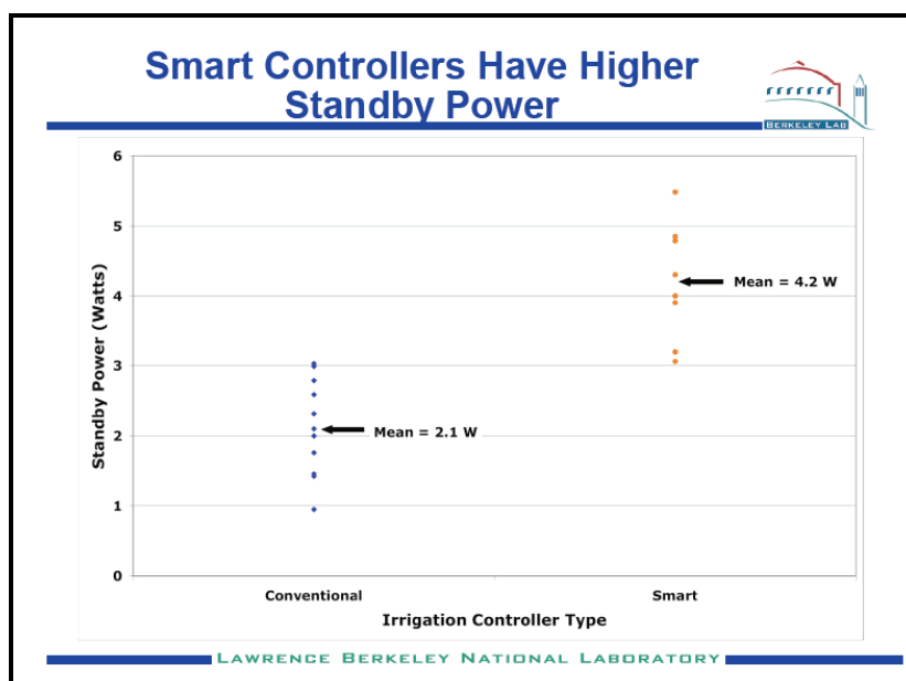
Figure 5. Standby Power Draw of Irrigation Controllers
