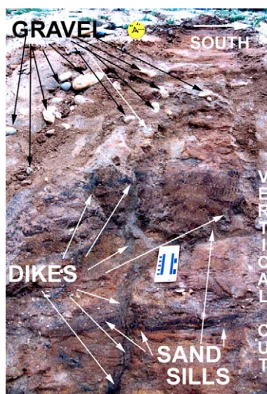
Fig. 16. Near-vertical exposure in a coastal terrace made for a major highway cut at Carlsbad, California (33.52–35.05 m el. MSL). Note: The gravel to boulder-bearing sands, deposited in a very fine, well-sorted dark mineral-rich matrix, are observed at the top of vents, and traceable to sand sills and dikes emanating from underlying marine source sands.
