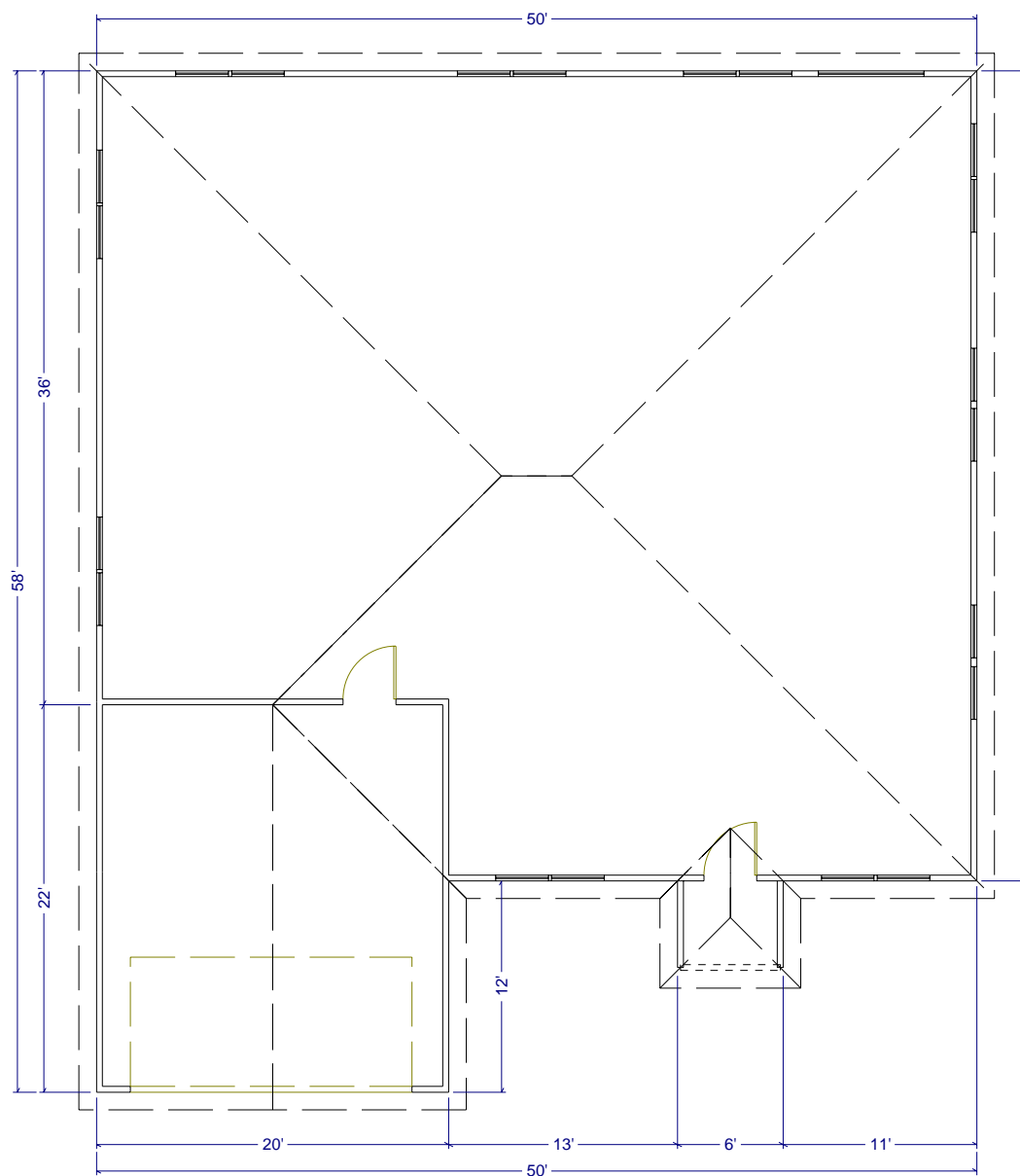
Figure 3 - One Story Prototype Floor Plan
