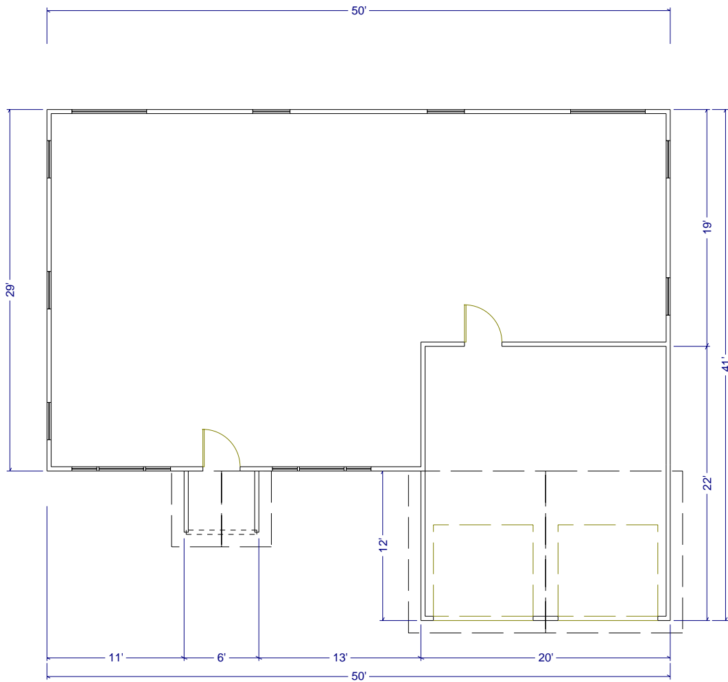
Figure 7 - Two Story Prototype Floor Plan – 2 nd Floor
