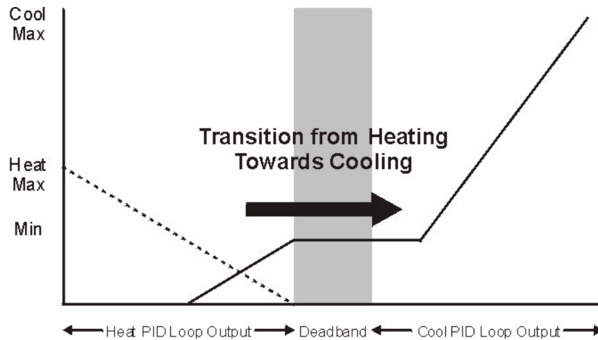
Figure 30. Dual Duct Mixing - From Heating to Cooling
