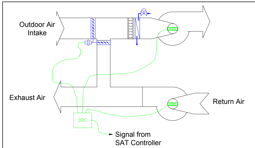
Figure 91. Return Fan Tracking
