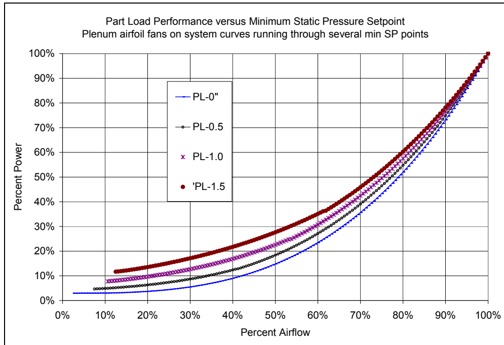
Figure 80. SP Setpoint vs Fan System Energy
