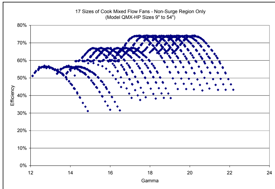
Figure 50. Gamma Curves for All Cook Airfoil Mixed Flow Fans
