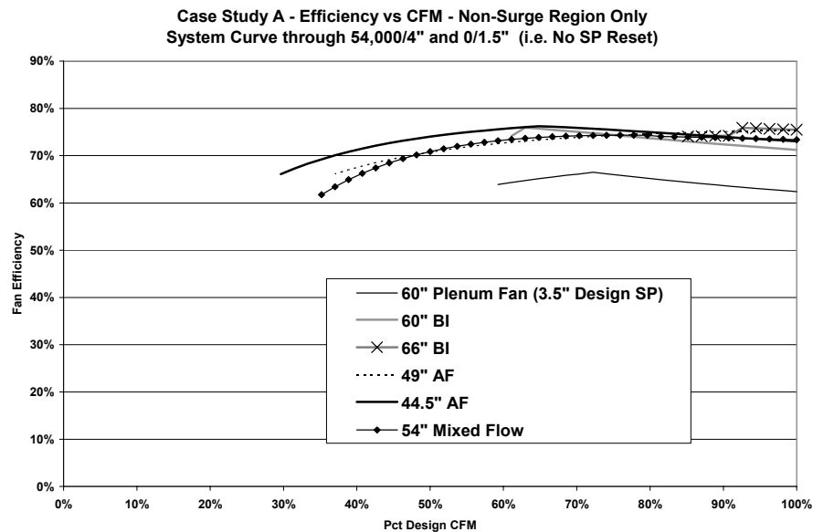
Figure 59. Case Study A - Part Load Efficiency (Non-surge Region Only)
