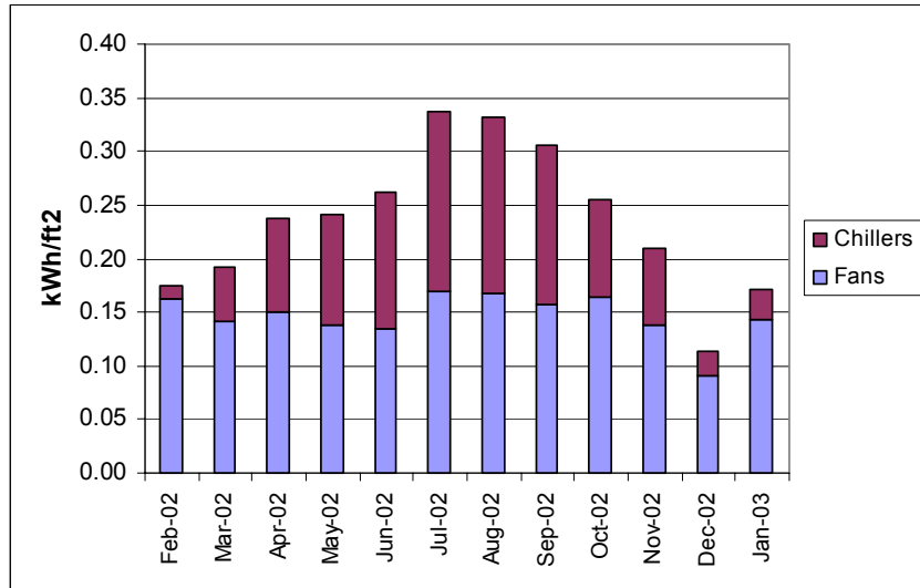
Figure 116. Comparison of Fan and Chiller Energy at Site 2 (Cumulative Graph, e.g. Combined Total is 0.34 kWh/ft 2 -yr in July)
