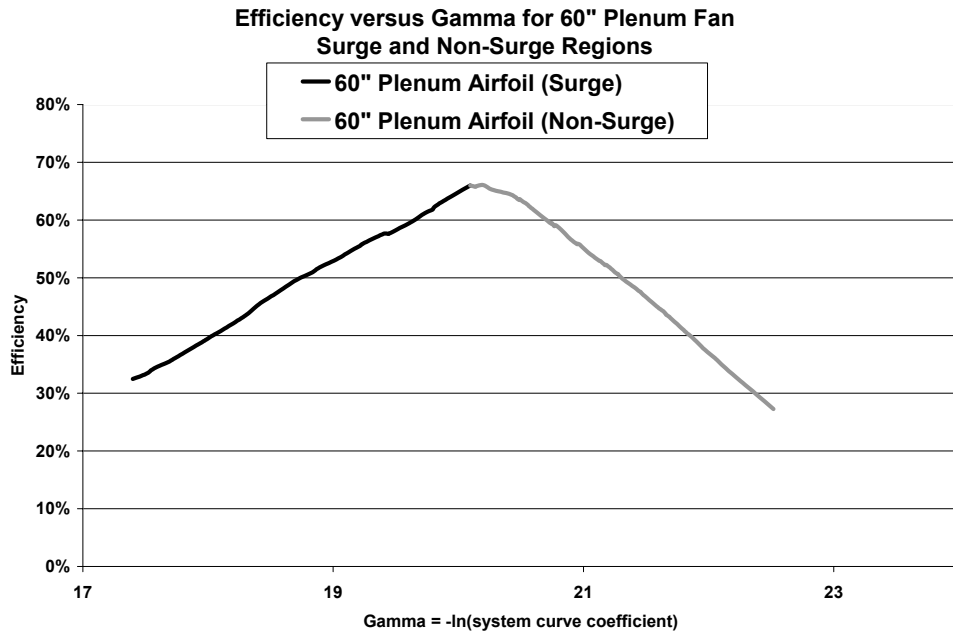
Figure 44. Gamma Curve
