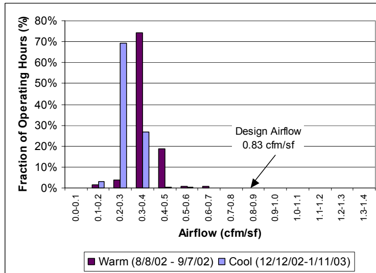
Figure 125. Total System Airflow, Site 3
