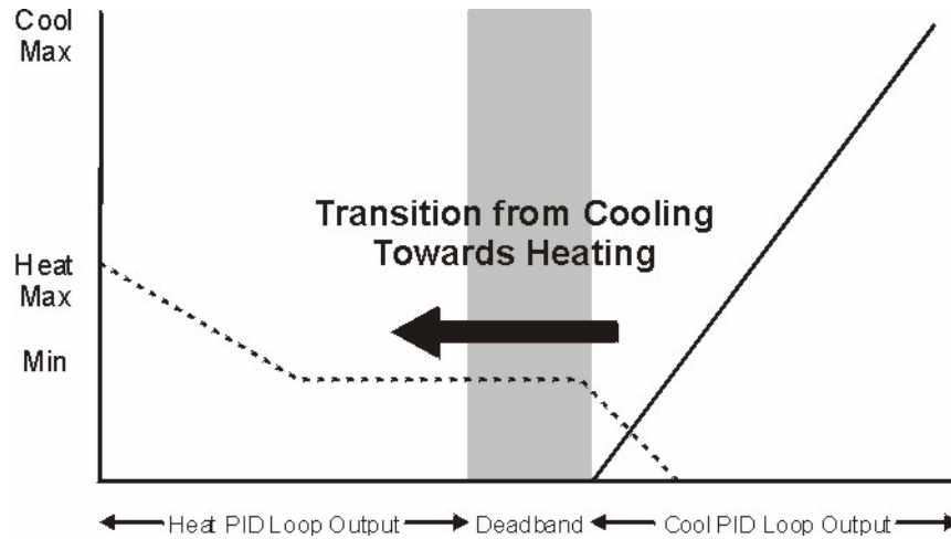
Figure 29. Dual Duct Mixing - From Cooling to Heating
