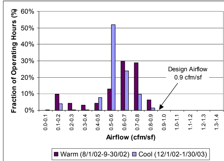
Figure 124. Total System Airflow, Site 2
