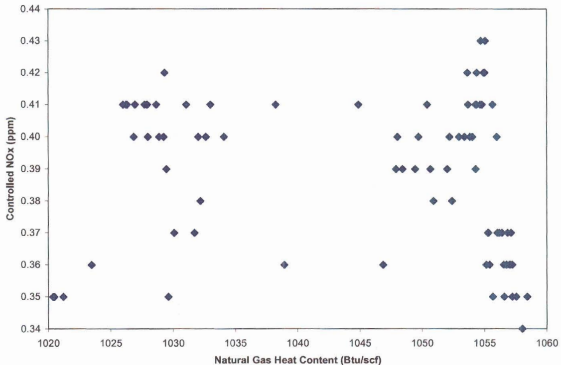
Figure 4-3: Redding Turbine Controlled NOx Concentration versus Natural Gas Heat Content
