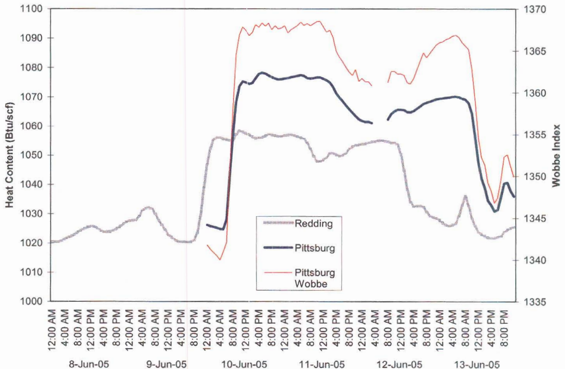
Figure 2-1: Pipeline Natural Gas Heat Content and Wobbe Index
