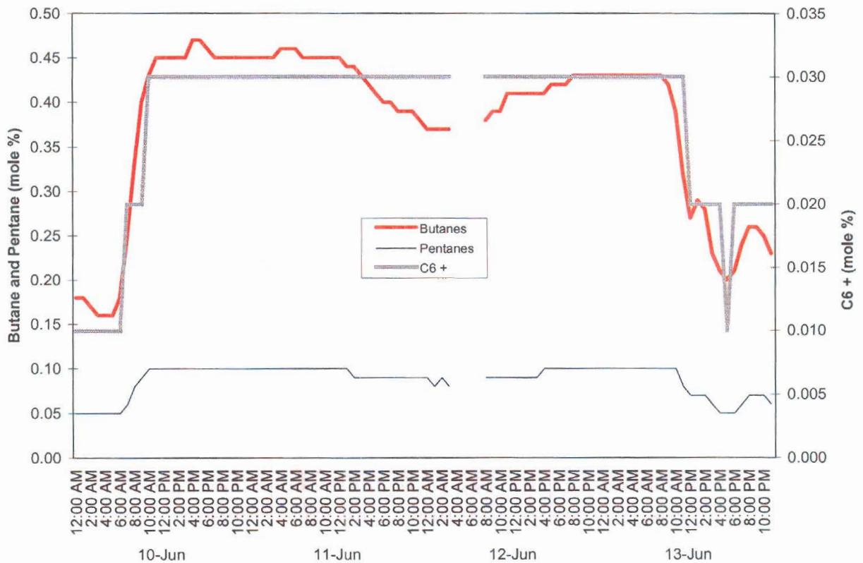
Figure 2-3: Pittsburgh Natural Gas Minor Component Composition
