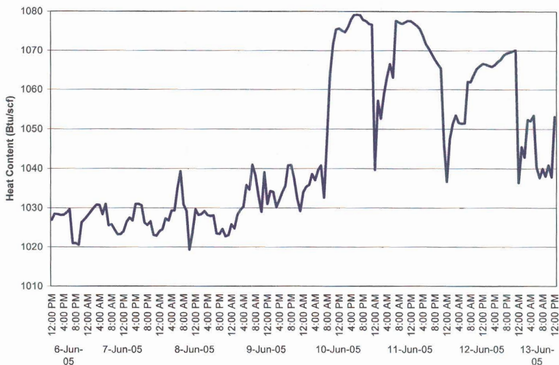
Figure 2-7: Los Medanos Natural Gas Heat Content Data
