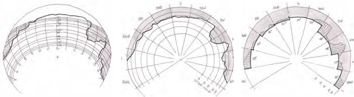
Figure 6 – Example Solar Access and Shading Analysis Instrument
