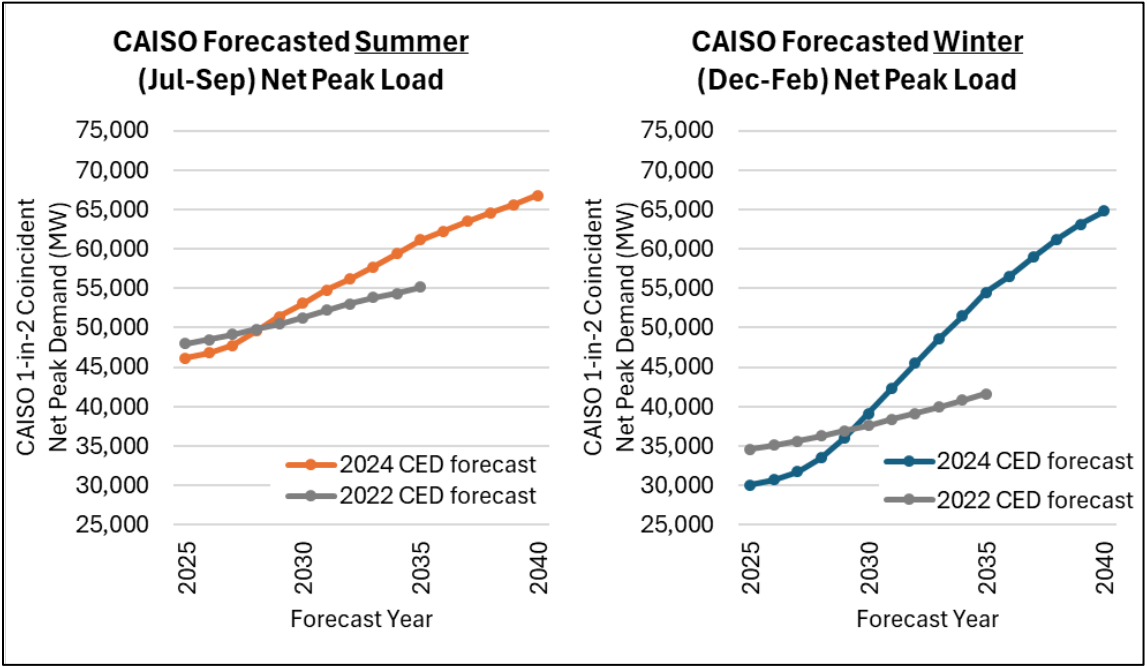
Figure 48: Statewide Coincident Peak Demand Forecast
