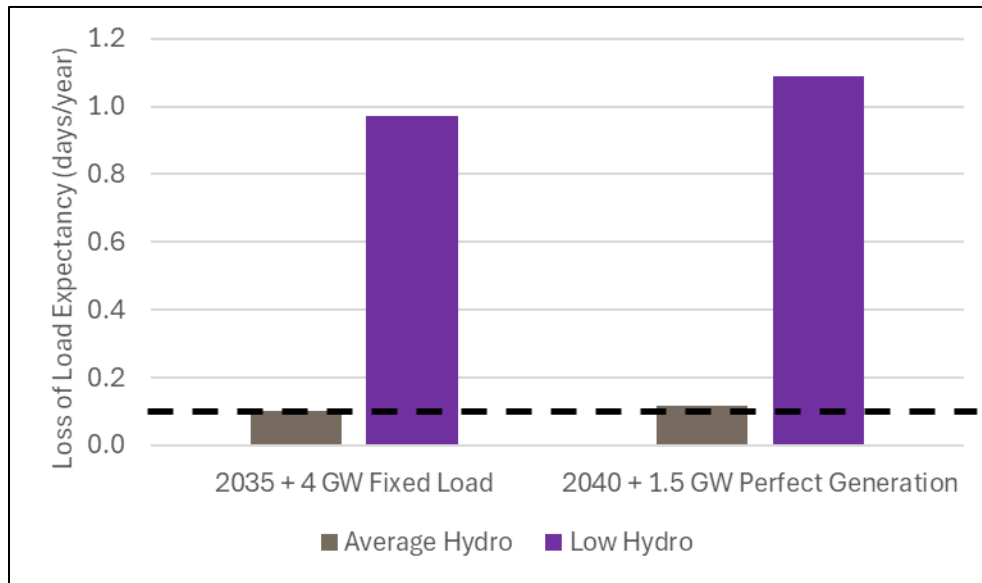
Figure 62: Loss of Load Expectancy for Average and Low Hydro Conditions
