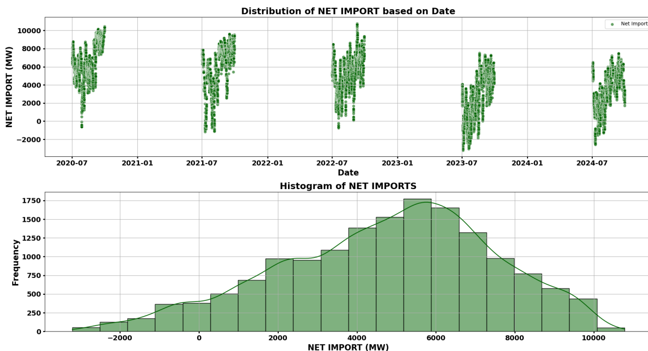
Figure 9: California ISO — Five-Year Summer Net Imports at Peak Hours
