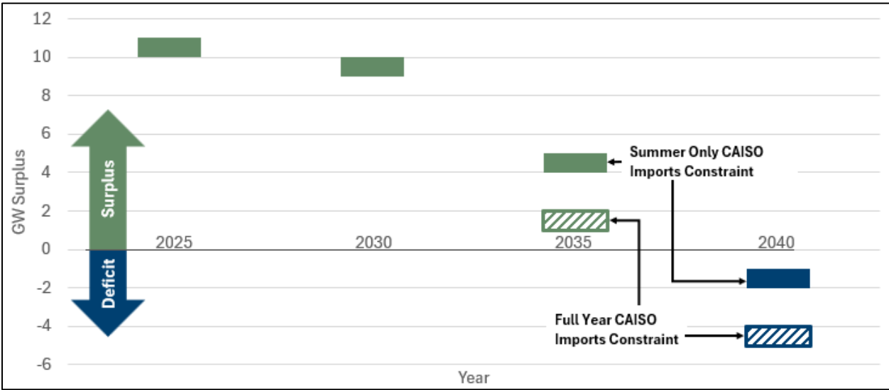
Figure 60: California Surplus Calculations given different CAISO Import Constraint Scenarios
