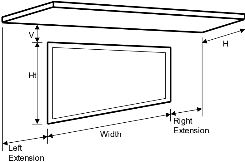
Figure 15: Overhang Dimensions
