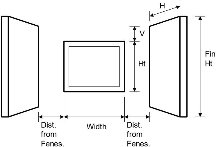
Figure 16: Sidefin Dimensions
