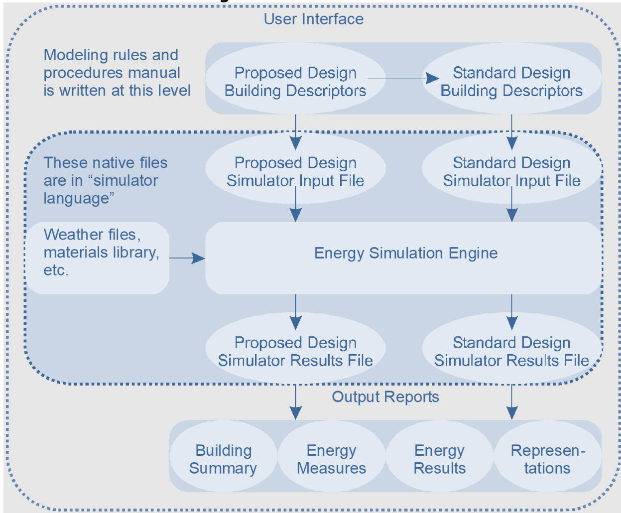
Figure 7: Information Flow
