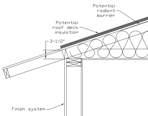
Figure 18: Section at Attic Edge with Standard Truss
