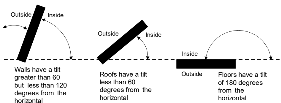
Figure 13: Surface Definitions
