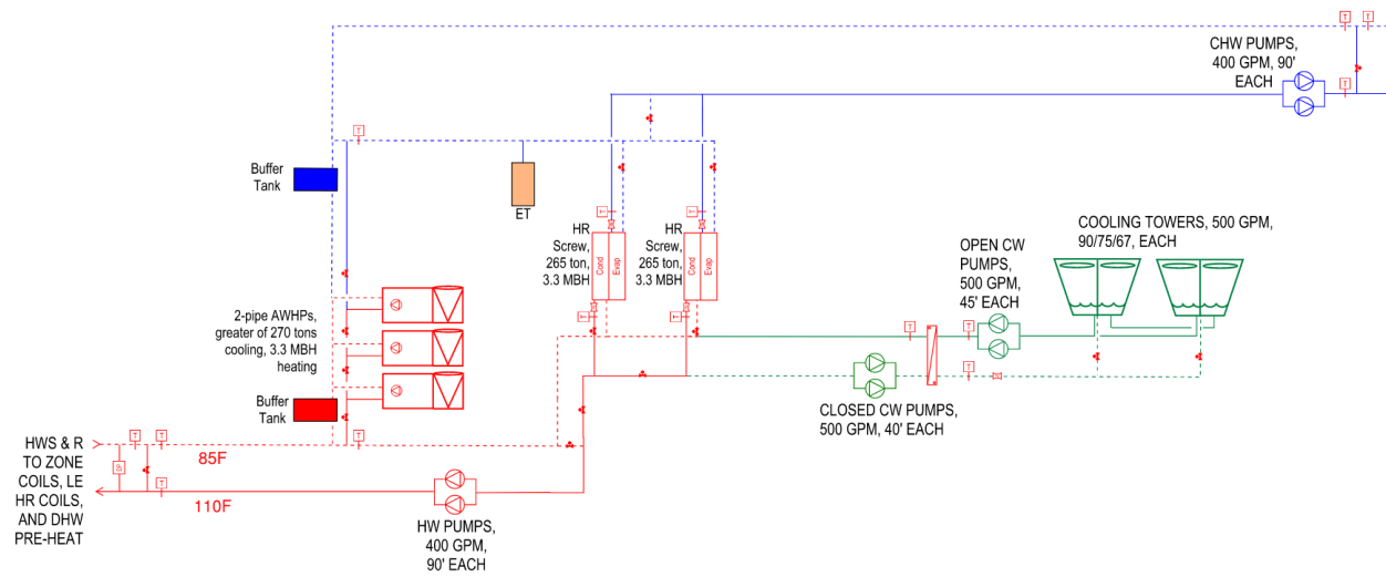
Figure 29. Piping Schematic of CHW Plant with Two Heat Recovery Chillers
