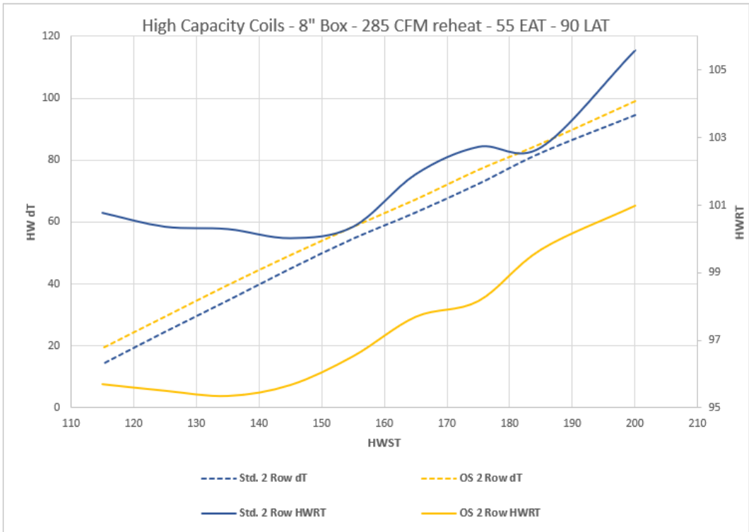
Figure 1: Typical VAV Box Coil Selections (55 EAT)
