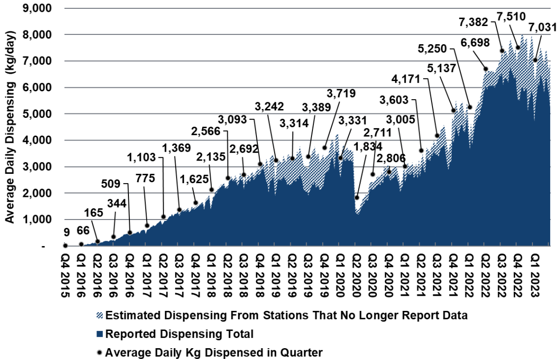
Figure D-1 shows the average daily dispensing of the network of hydrogen stations from the fourth quarter of 2015 to the first quarter of 2023. The chart also shows estimated dispensing for stations that no longer report dispensing data to the CEC.
