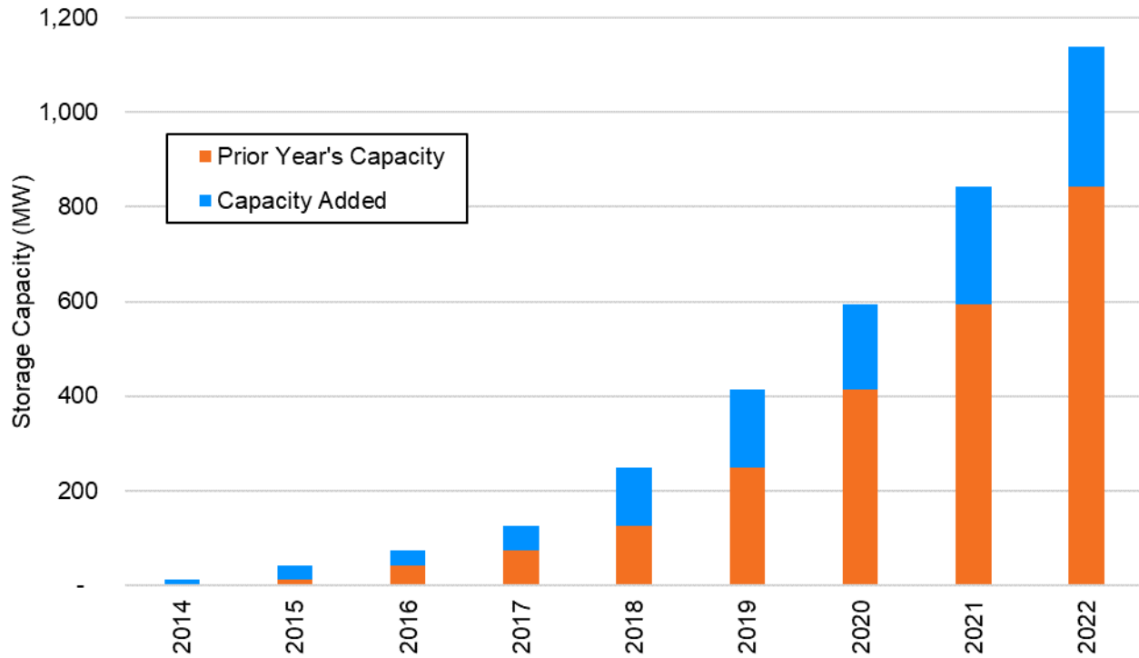
Figure 18: Cumulative BTM Storage Capacity in California
