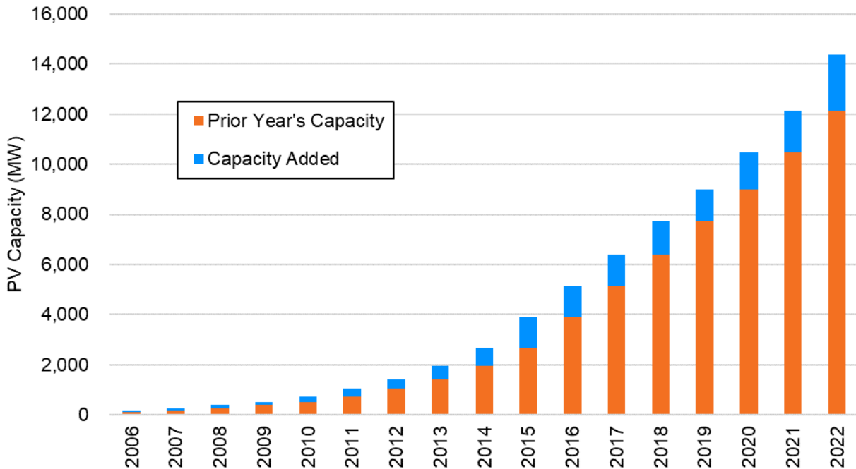
Figure 17: Cumulative BTM PV Capacity in California
