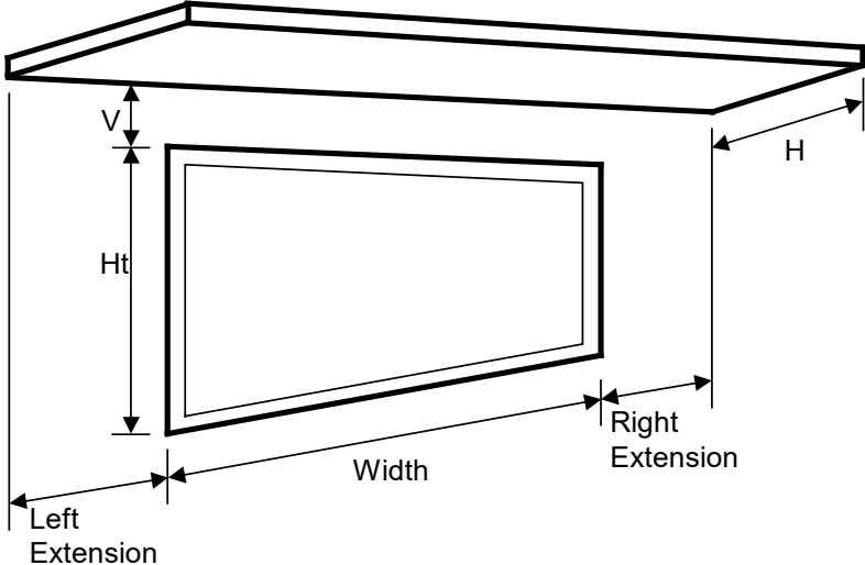
Figure 14: Overhang Dimensions
