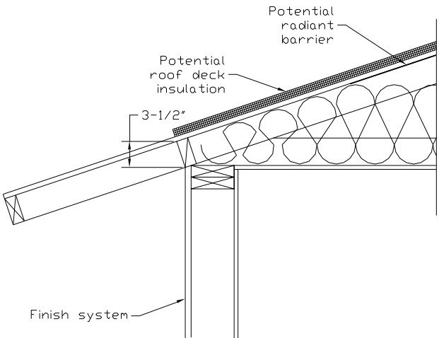
Figure 17: Section at Attic Edge with Standard Truss
