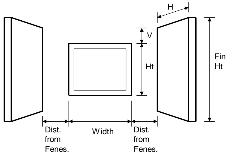
Figure 15: Sidefin Dimensions
