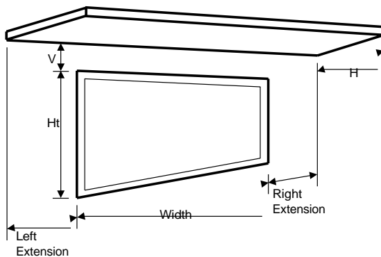
Figure 14: Overhang Dimensions
