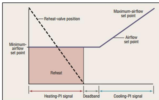
Figure 9: Single Maximum VAV Box Control
