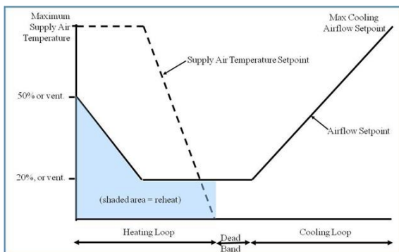
Figure 10: Dual Maximum Control Sequence
