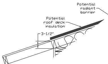
Figure 17: Section at Attic Edge with Standard Truss
