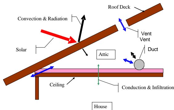
Figure 16: Attic Model Components
