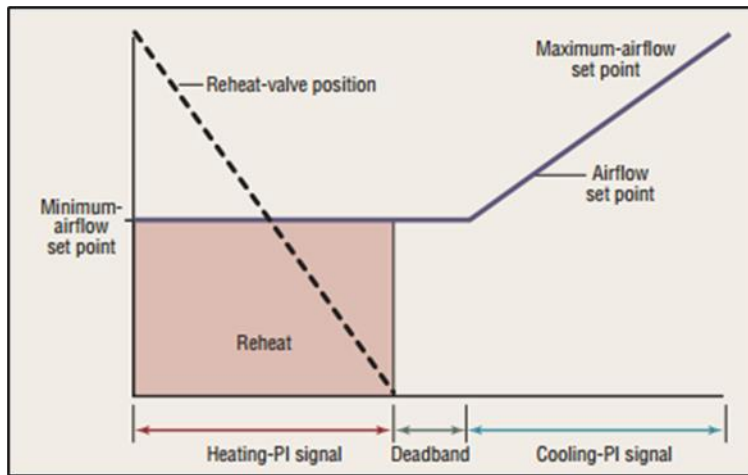
Figure 9: Single Maximum VAV Box Control
