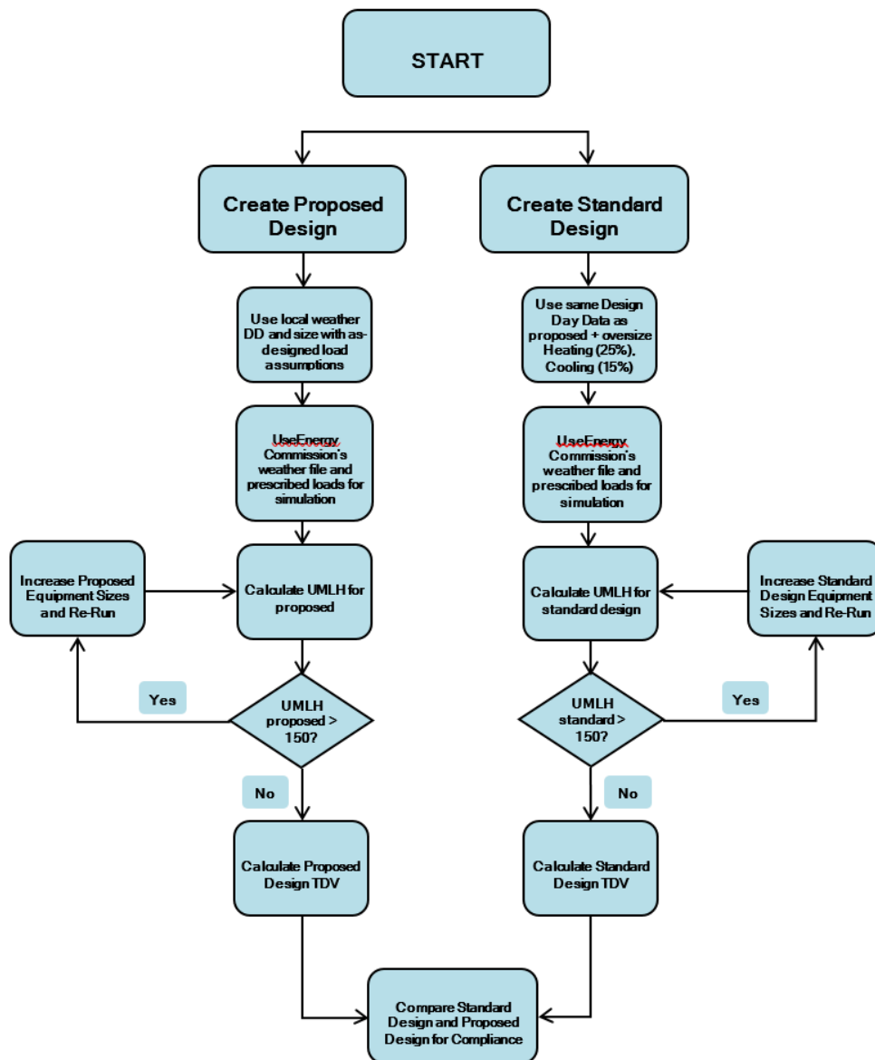
Figure 2: Calculation Process for Title 24 Compliance
