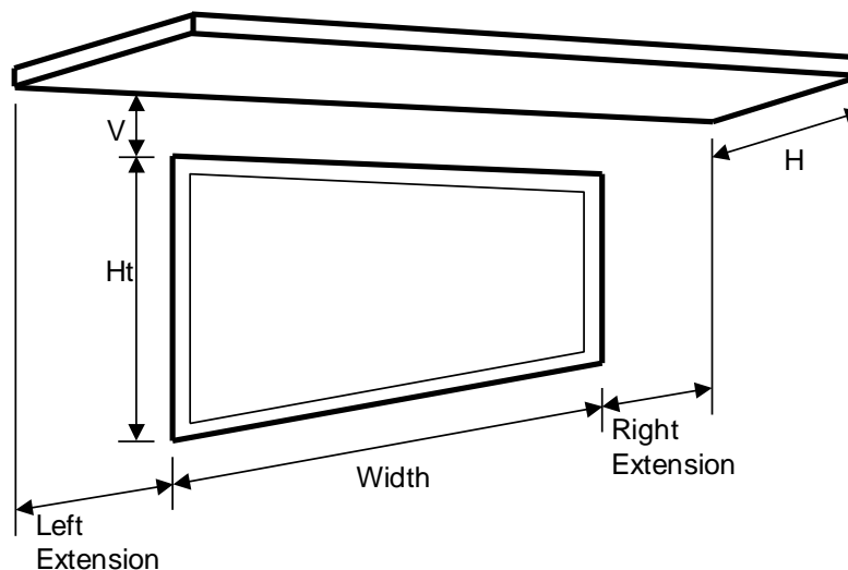
Figure 14: Overhang Dimensions
