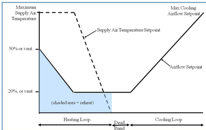
Figure 10: Dual Maximum Control Sequence
