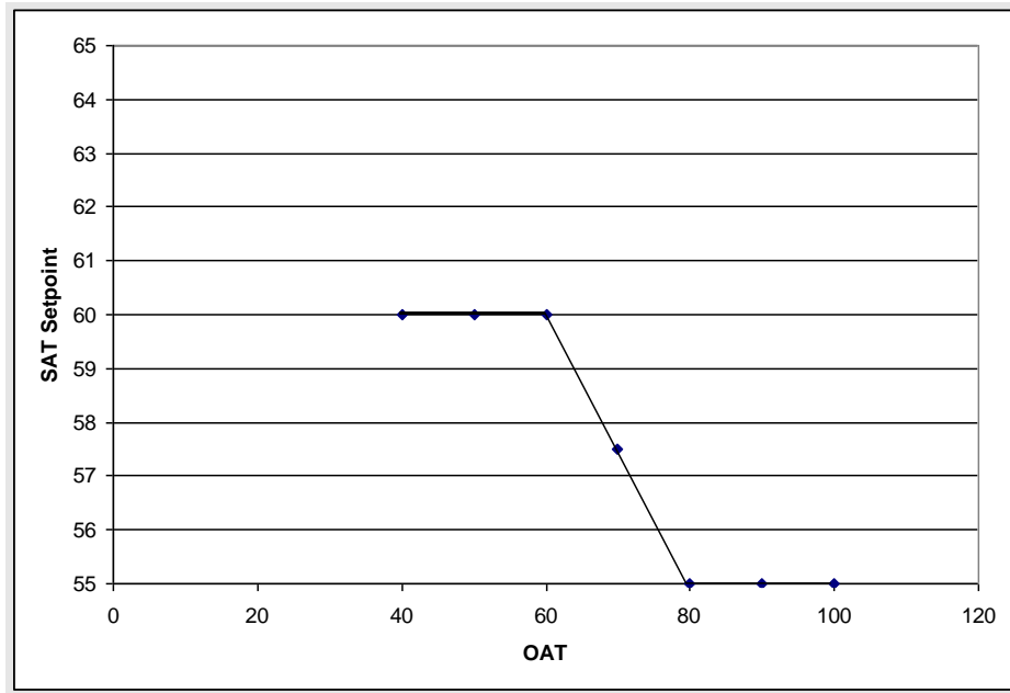
Figure 8: SAT Cooling Setpoint Reset Based on Outdoor Air Temperature (OAT)
