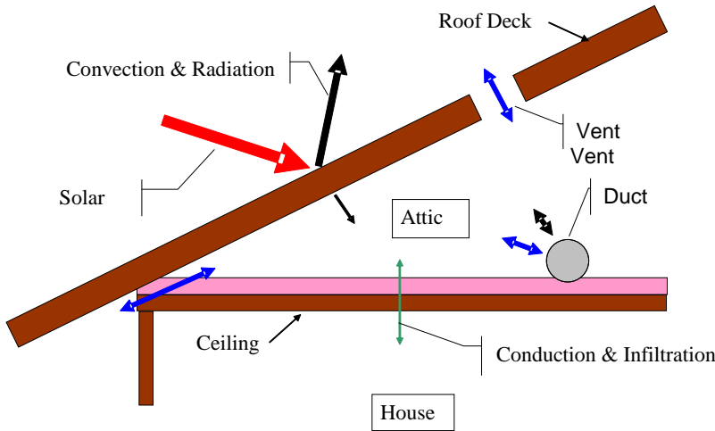
Figure 16: Attic Model Components
