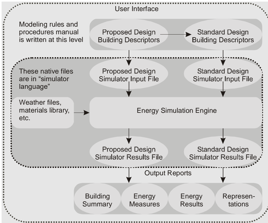
Figure 7: Information Flow
