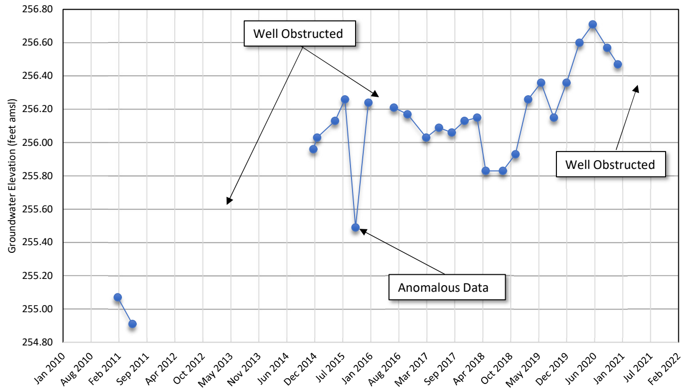
Chart 8 County Well 36G1S Hydrograph
