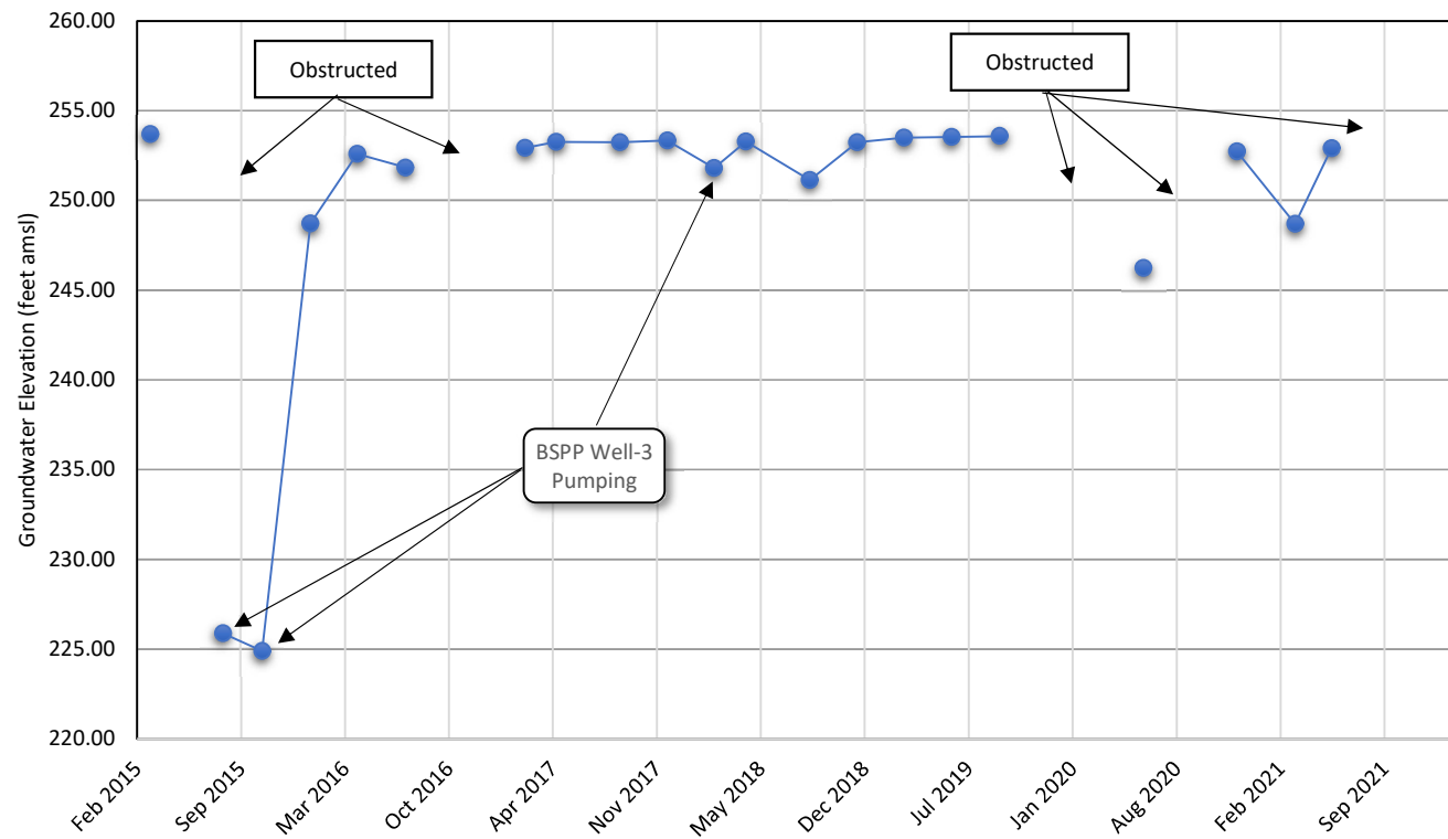
Chart 3 BSPP Well-3 Hydrograph
