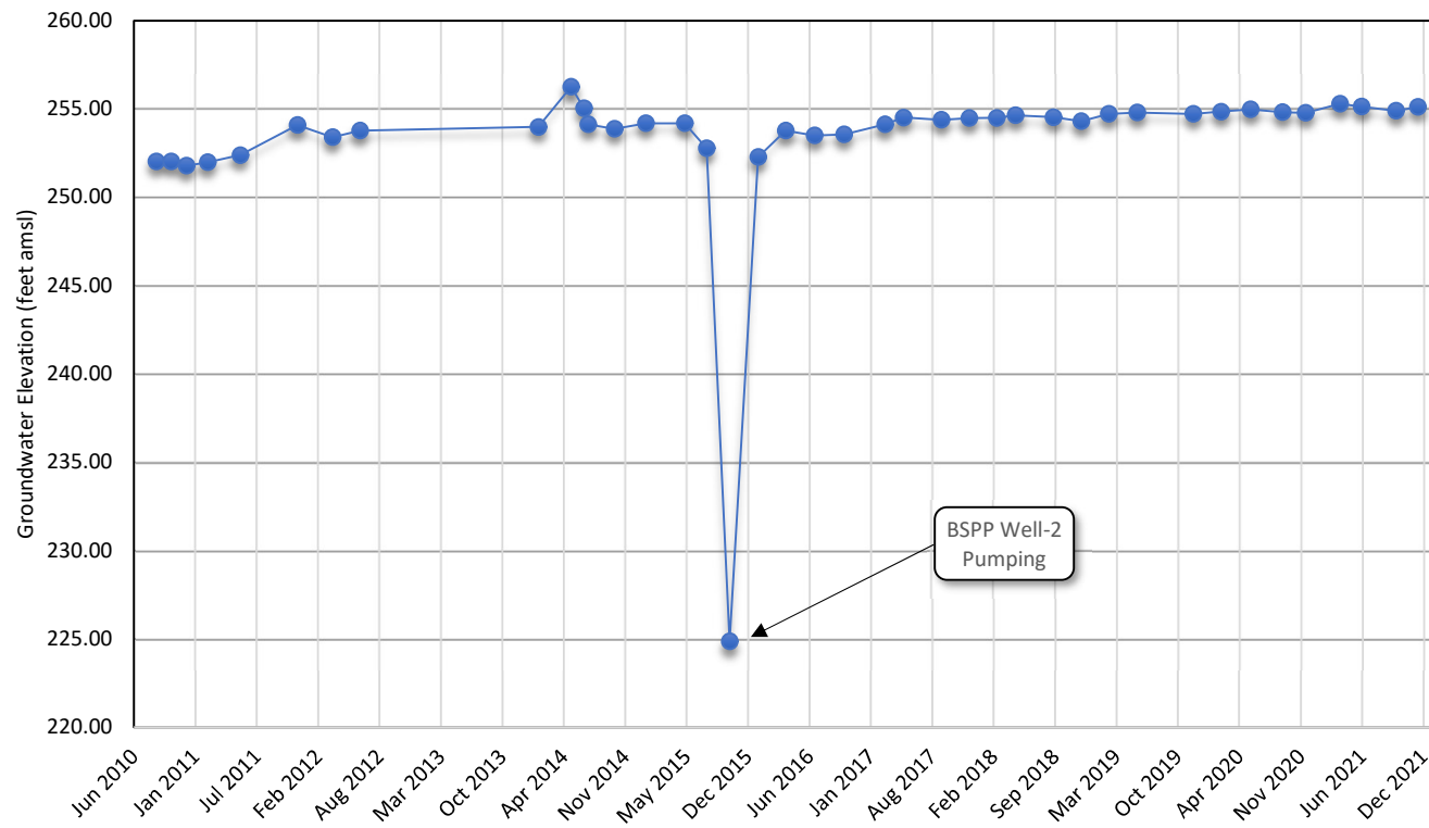
Chart 1 BSPP Well-2 Hydrograph
