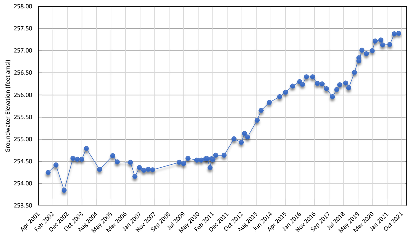
Chart 10 6S/22E-09P1S Well Hydrograph
