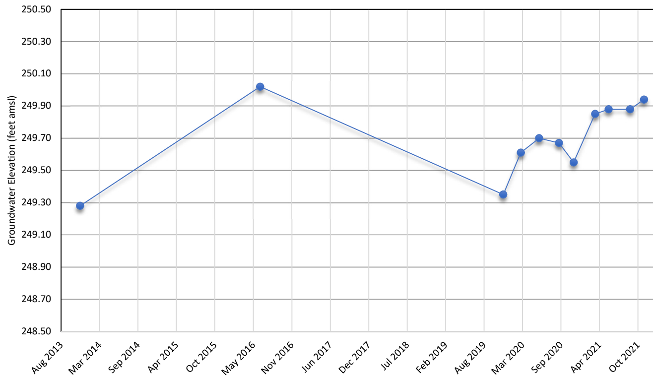
Chart 11 6S/22E-19N2S Well Hydrograph
