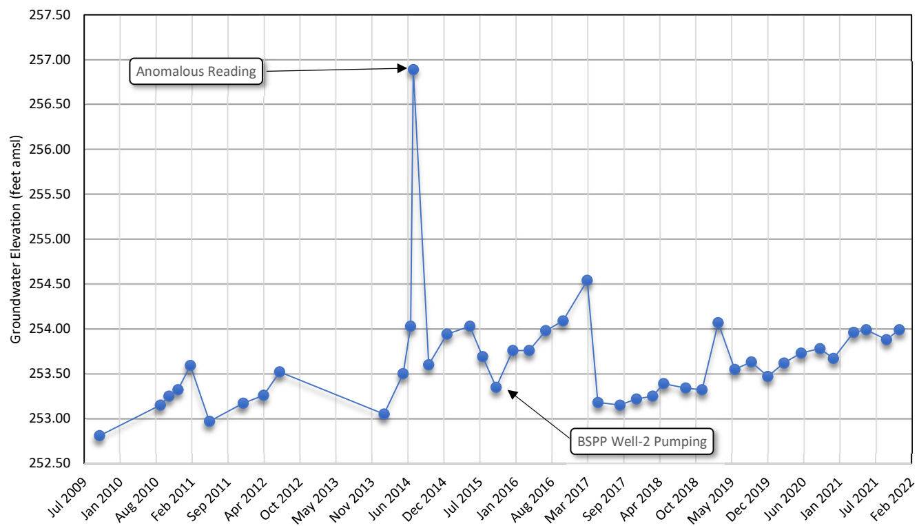
Chart 2 BSPP WO-2 Hydrograph
