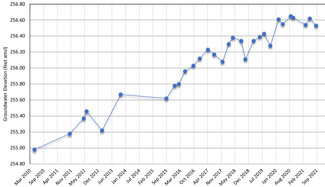
Chart 9 5S/22E-31E1S Well Hydrograph
