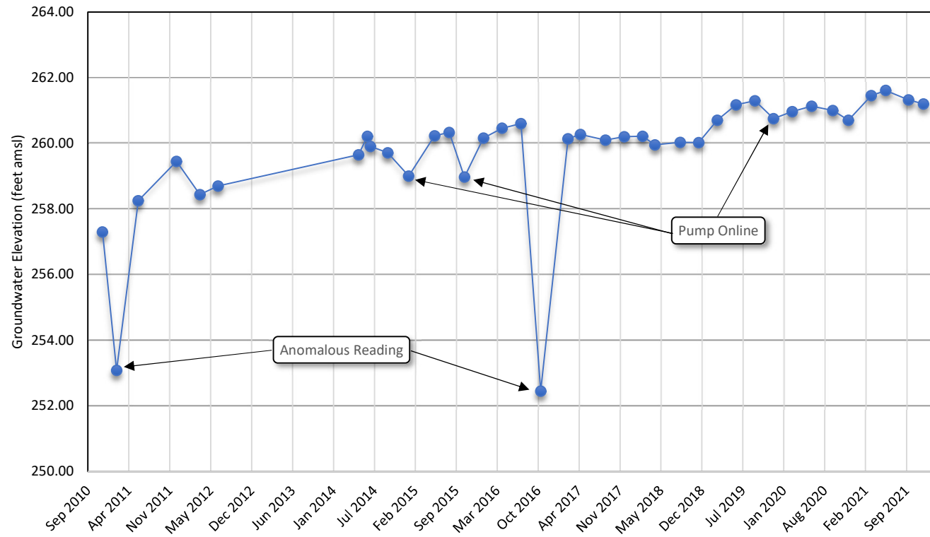
Chart 4 Gila Farm Well Hydrograph
