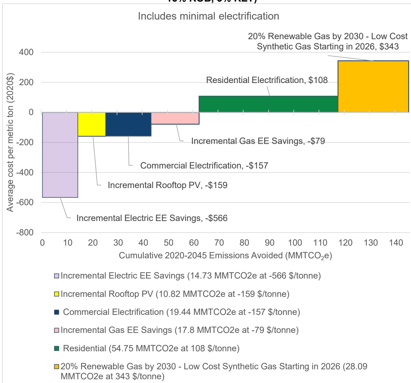
Figure C- 57: Aggregated Marginal Abatement Cost Curve Using Scenario 6.a (100% NC, 15% ROB, 5% RET)
