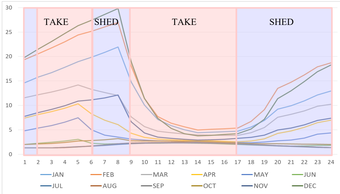
Figure C-21: Scenario 6 Commercial Space Heating
