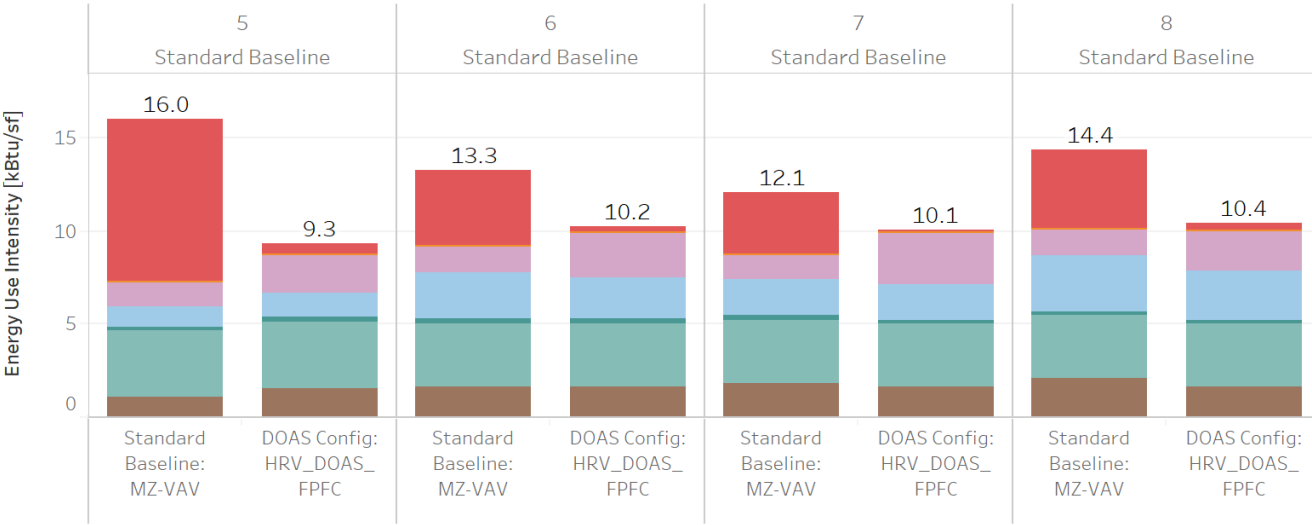
Site Energy Use Intensity [kBtu/sf] | SecondarySchool | Climate Zones 5, 6, 7 and 1 more
