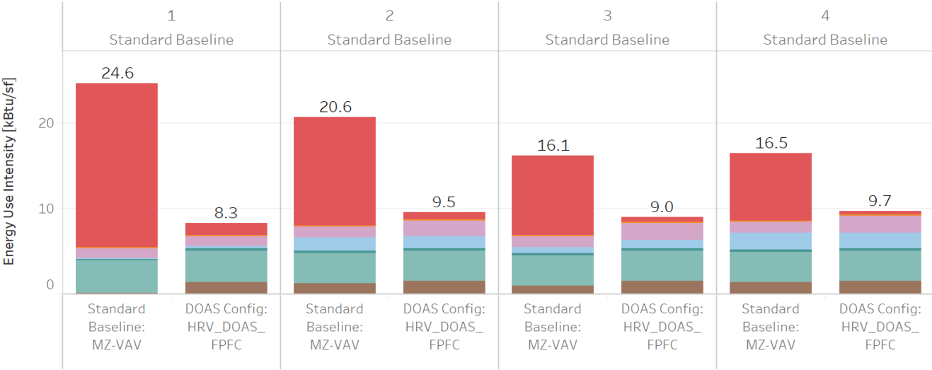
Site Energy Use Intensity [kBtu/sf] | SecondarySchool | Climate Zones 1, 2, 3 and 1 more
