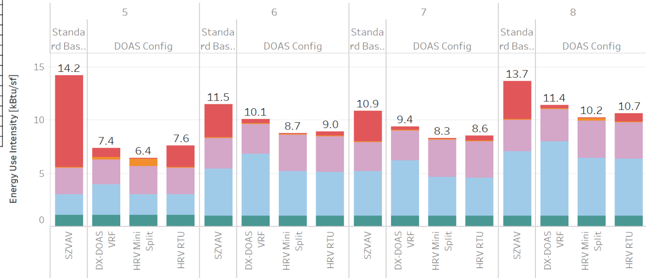
Site Energy Use Intensity [kBtu/sf] | OfficeSmall | Climate Zones 5, 6, 7 and 1 more
