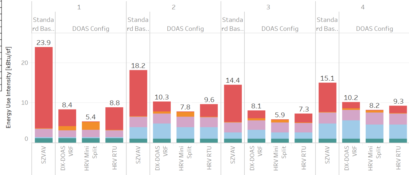
Site Energy Use Intensity [kBtu/sf] | OfficeSmall | Climate Zones 1, 2, 3 and 1 more
