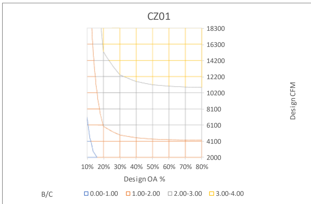
Figure 52: Cost effectiveness of EAHR in CZ1 with 8,760 hours of operation.
