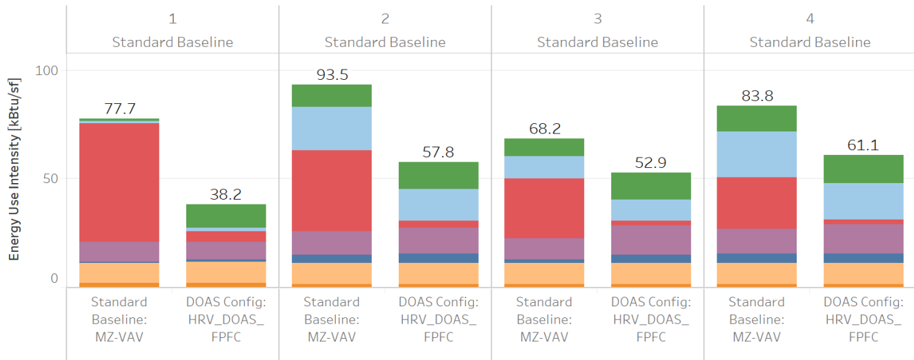
TDV HVAC Energy Use [kTDV/sf] | SecondarySchool | Climate Zones 1, 2, 3 and 1 more
