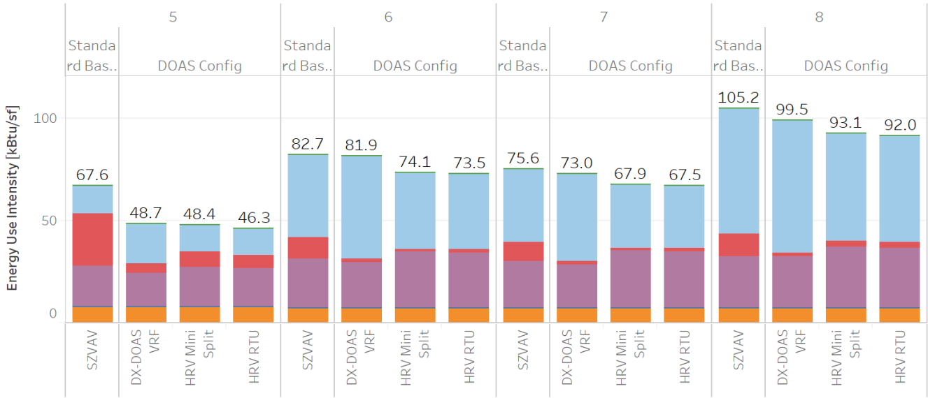
TDV HVAC Energy Use [kTDV/sf] | OfficeSmall | Climate Zones 5, 6, 7 and 1 more
