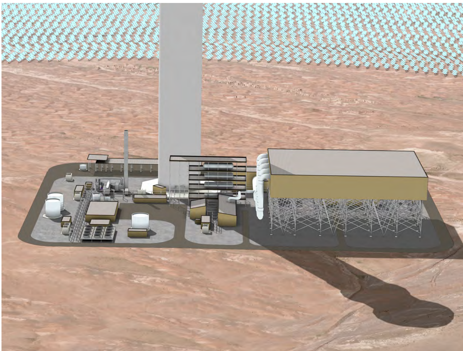
TYPICAL VIEW OF POWER BLOCK FROM THE SOUTH FACING NORTH RIO MESA SOLAR ELECTRIC GENERATING FACILITY
