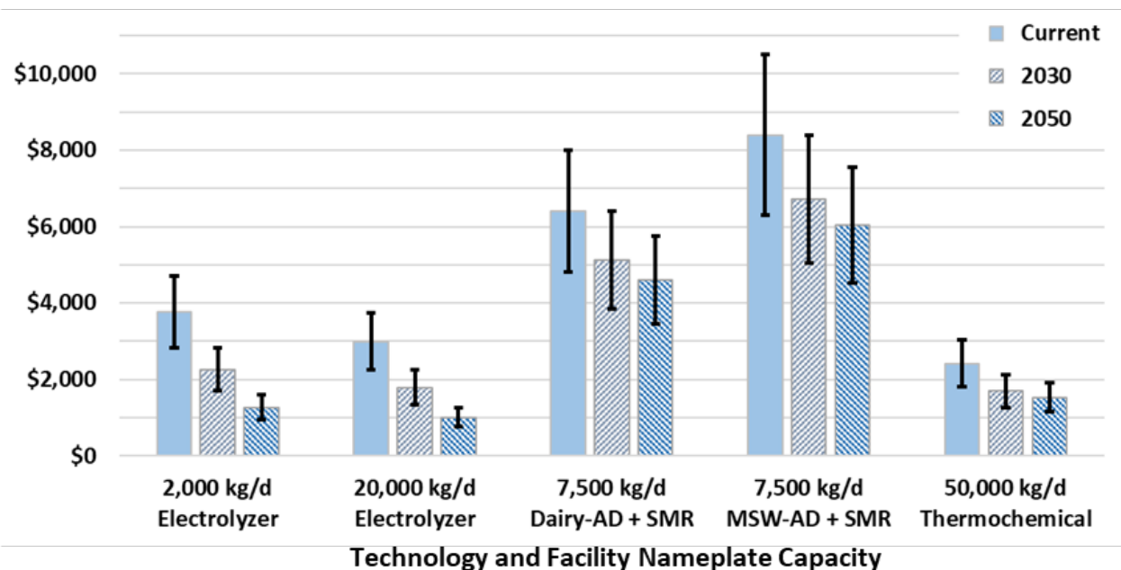
Figure 22: Capital Cost per Unit of Renewable Hydrogen Production Capacity
