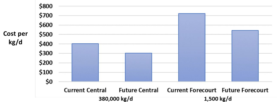
Figure A-20: Current and Future Steam Methane Reformation Capital Costs
