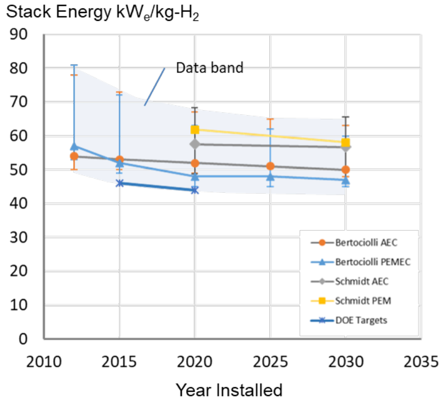
Figure A-11: Electrolyzer Conversion Efficiency Forecasts
