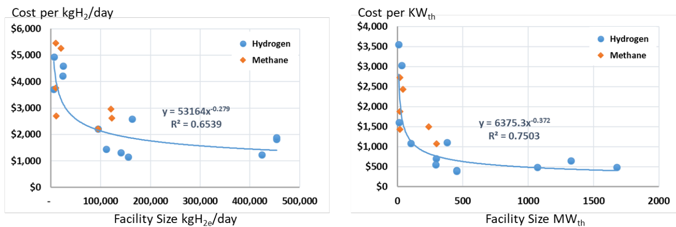
Figure A-24: Gasification System Capital Costs
