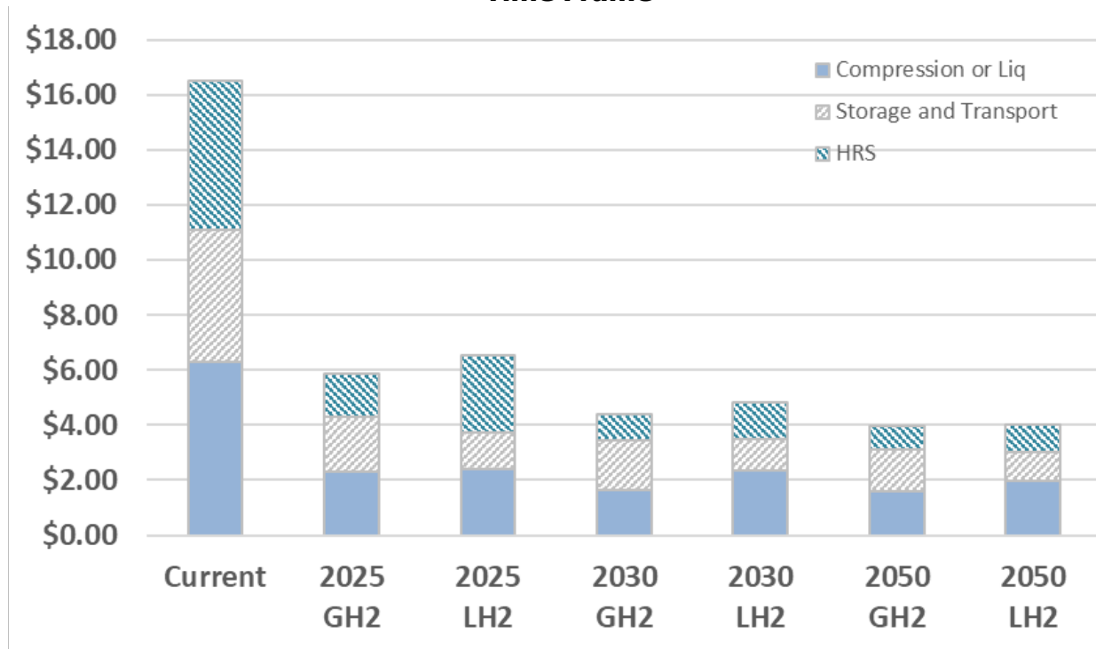
Figure 30: Plant-Gate-to-Dispenser Cost per Kilogram of Hydrogen by Mode and Time Frame
