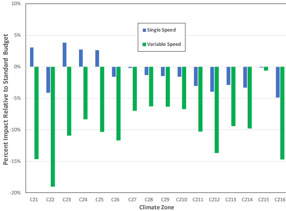
Figure 1: Single and variable speed AWHP compliance impacts (2019)
