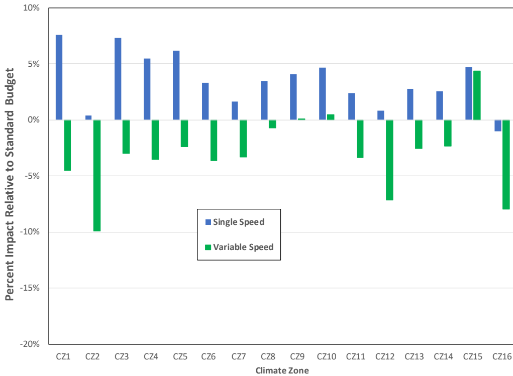
Figure 2: Single and variable speed AWHP impacts (2019, Ducts in Conditioned Space)
