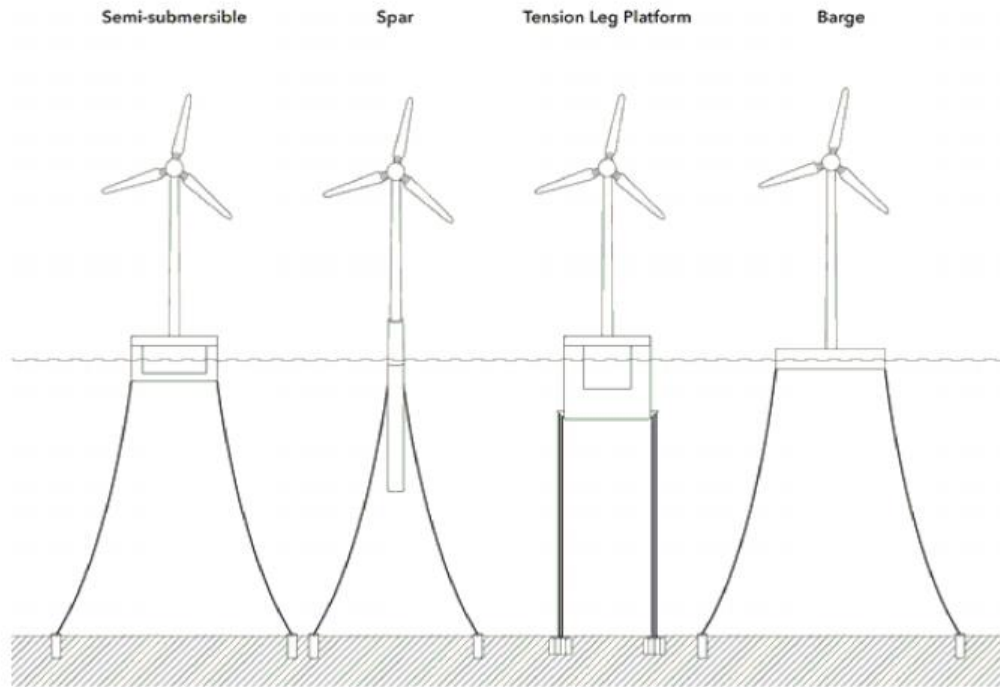
Figure illustrates four types of floating offshore wind platform designs: semisubmersible, spar, tension leg platform, and barge.
