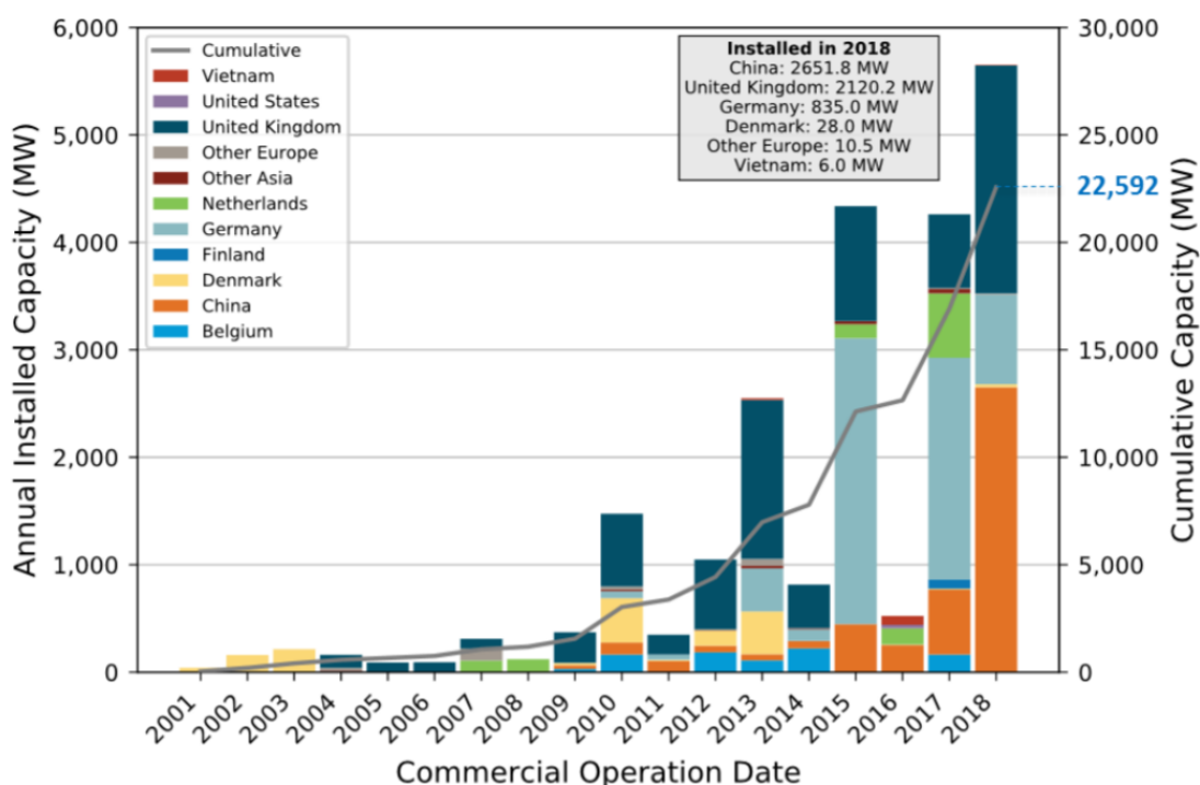
Figure 4: Global Offshore Wind Installed Capacity by Year: 2001-2018
