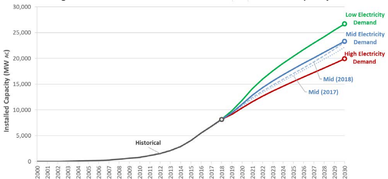
Figure 31: Statewide Behind-the-Meter Photovoltaic Capacity
