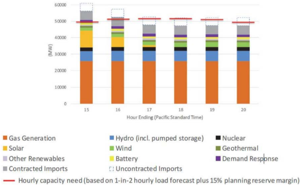
Figure 8: 2021 Projected Energy Production from Resource Adequacy Fleet
