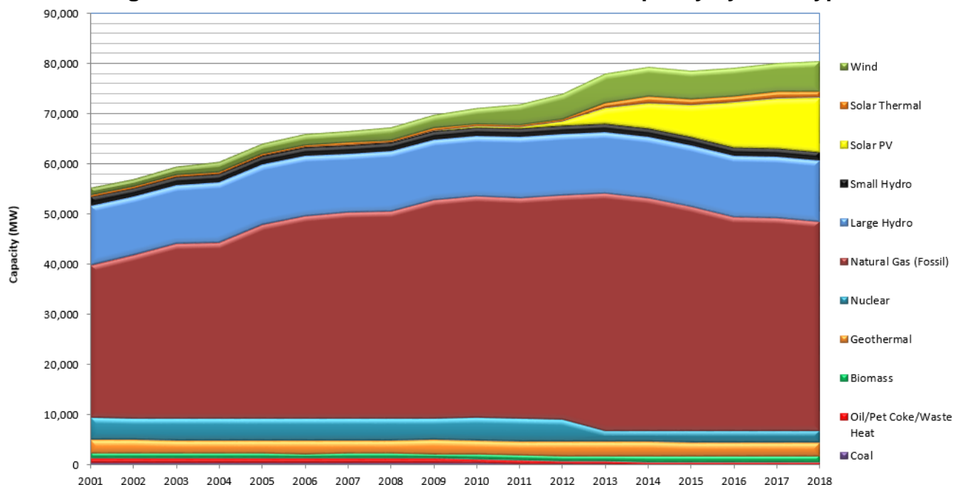
Figure 3: Installed In-State Electric Generation Capacity by Fuel Type
