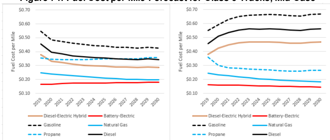
Figure 74: Fuel Cost per Mile Forecast for Class 6 Trucks, Mid Case
