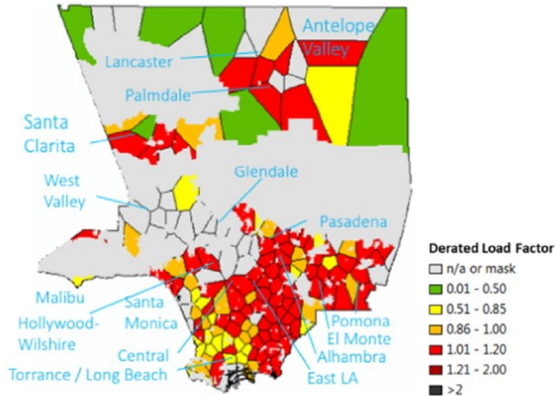
Figure 24: Map of SCE Substation Vulnerabilities to Heat Waves in 2018
