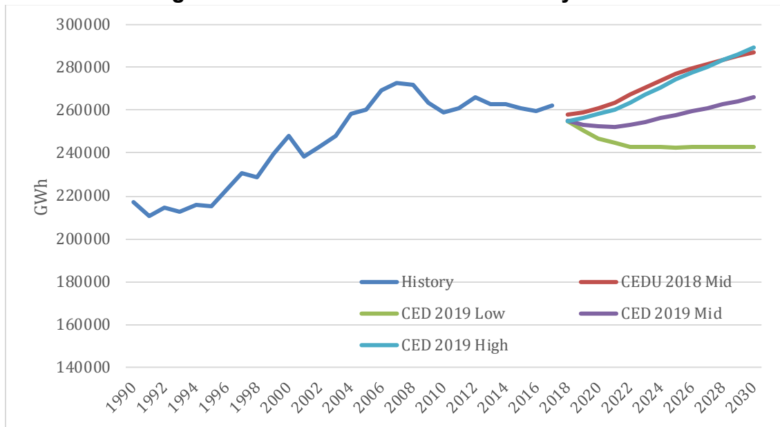
Figure 32: Statewide Baseline Electricity Sales
