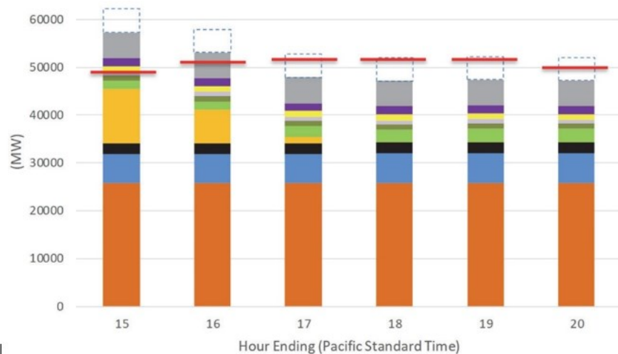
Figure 9: 2022 Projected Energy Production from Resource Adequacy Fleet
