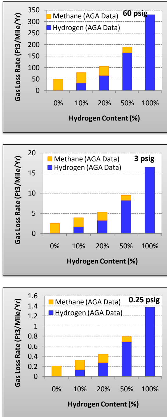
Figure 9. The Calculated Gas Loss Rate vs. Hydrogen Concentration in Hydrogen/Methane Mixtures at the Typical Distribution Operating Pressures (60 psig (4.1 bar), 3 psig (210 mbar) and 0.25 psig (17.2 mbar))*
