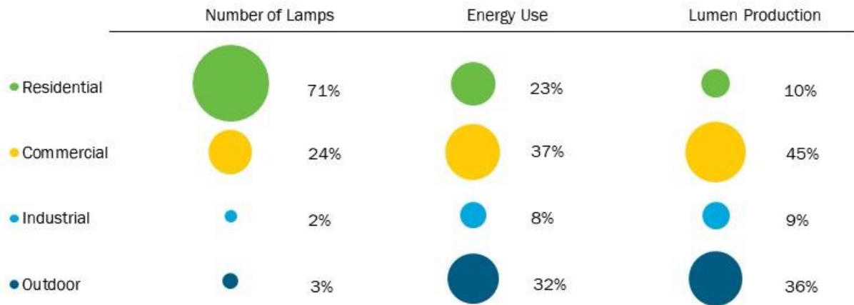
Figure 5.2 U.S. Lighting 41 Inventory, Electricity Consumption and Lumen Production in 2015
