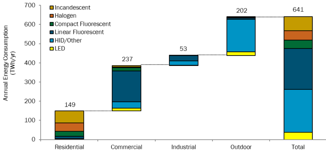
Figure 5.3 U.S. Lighting Electricity Consumption by Sector and Technology Type in 2015
