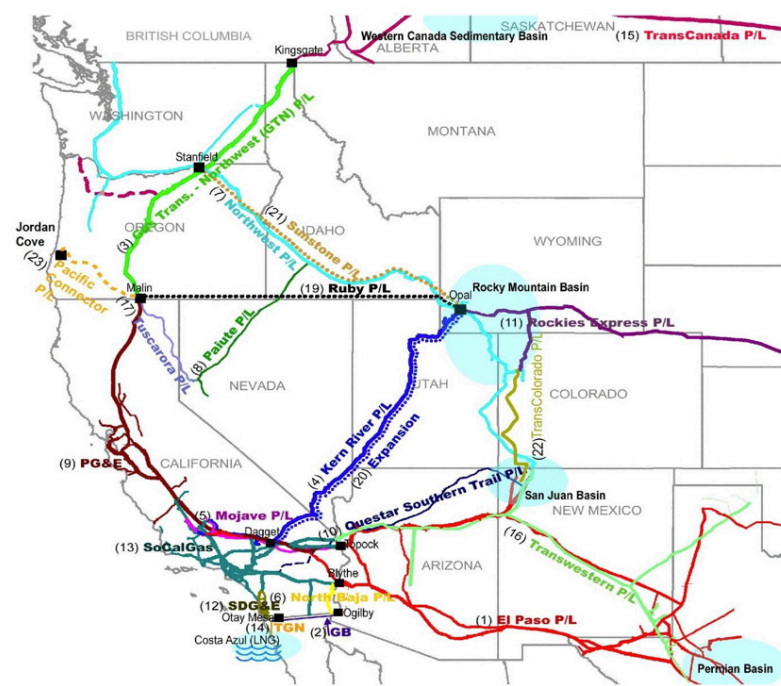
Figure 70: Western North American Natural Gas Pipelines
