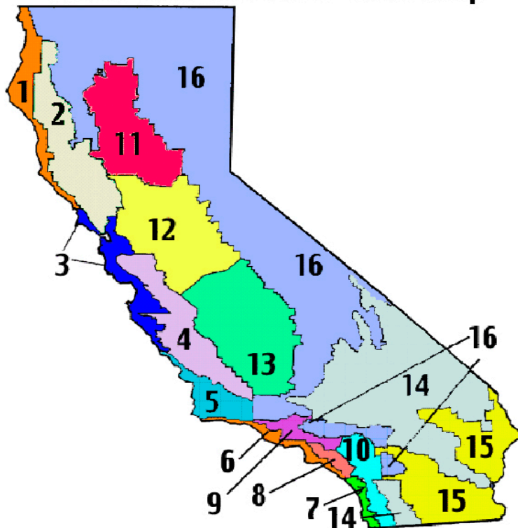
California Climate Zone Map
