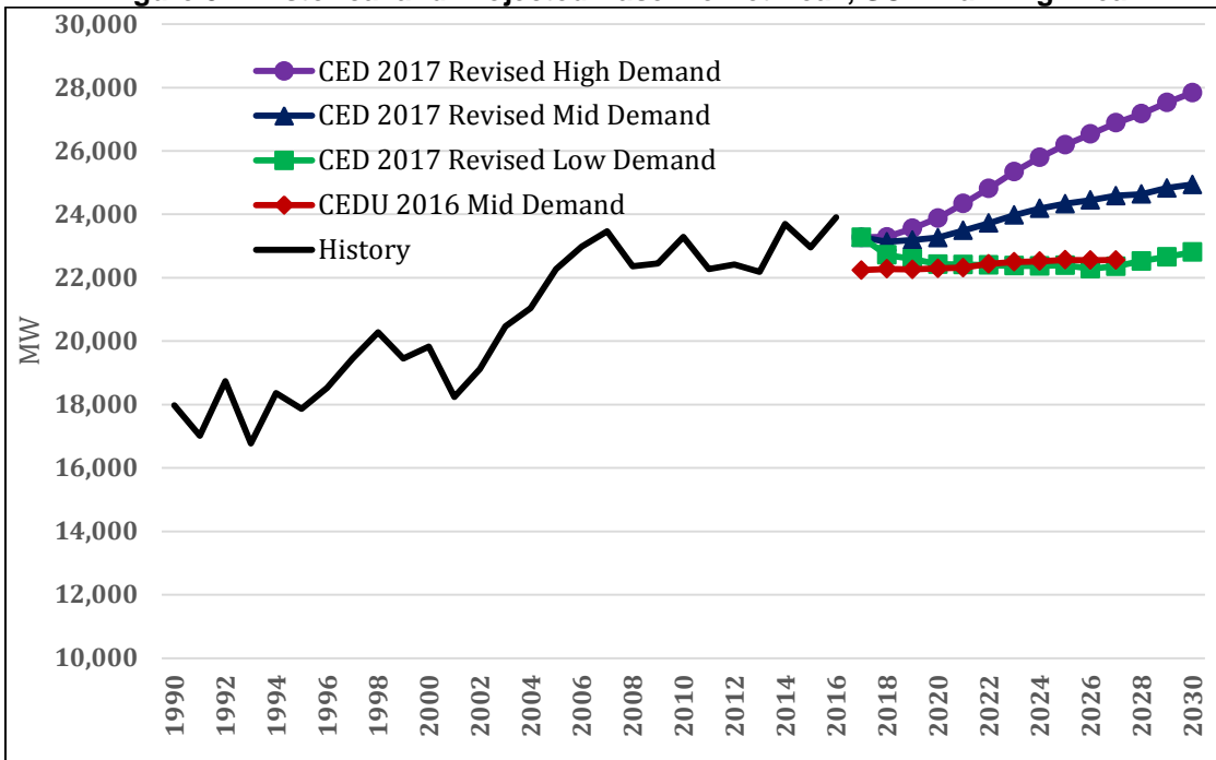
Figure 52: Historical and Projected Baseline Net Peak, SCE Planning Area
