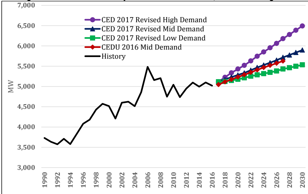
Figure 62: Historical and Projected Baseline Net Peak, NCNC Planning Area
