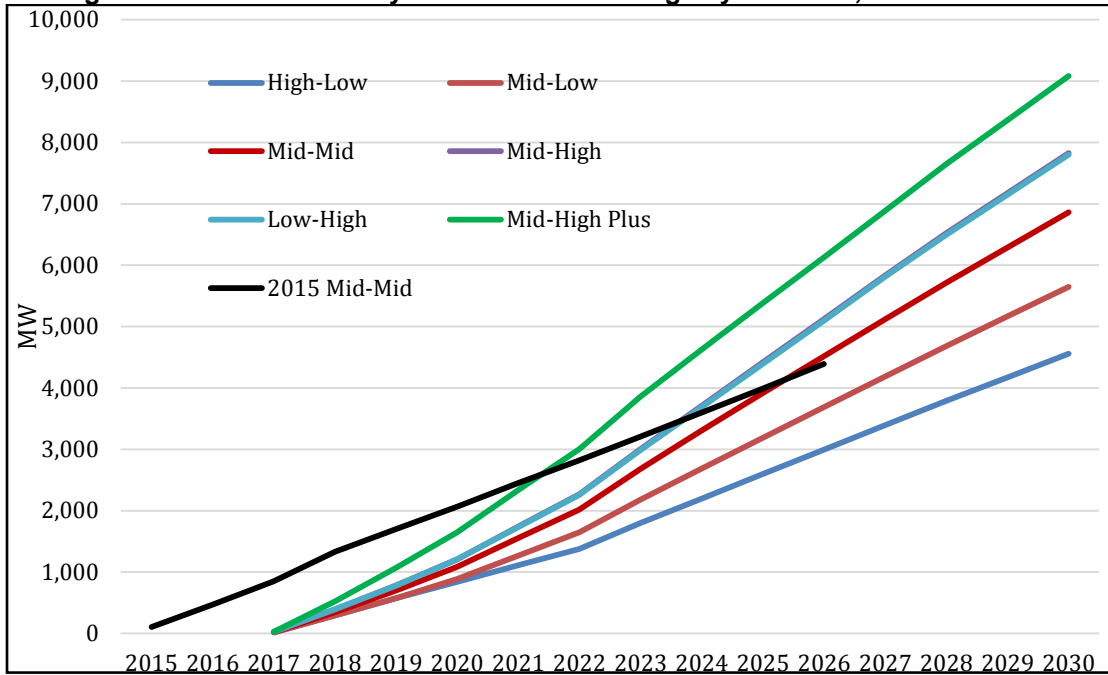
Figure 26: AAE Electricity Peak Demand Savings by Scenario, Combined IOUs
