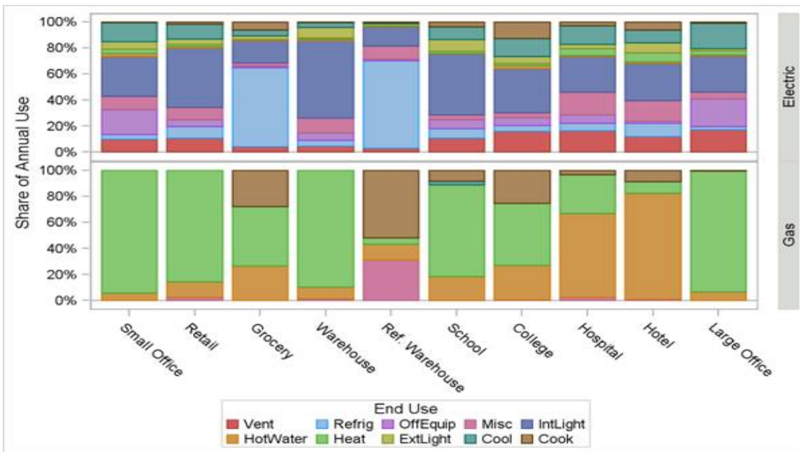
Figure A-6: Distribution of Annual End-Use Consumption by Fuel Type – North Coastal Small/Medium Buildings
