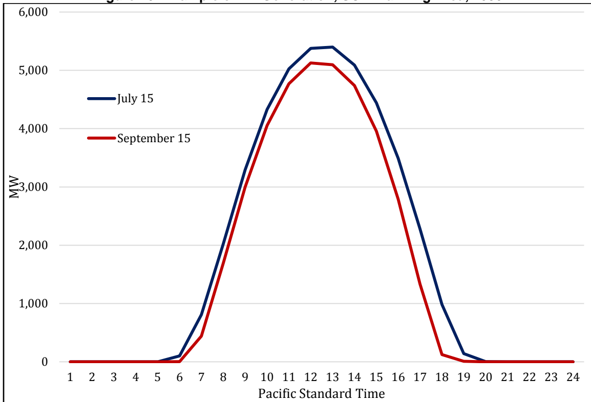
Figure 40: Example of PV Generation, SCE Planning Area, 2030
