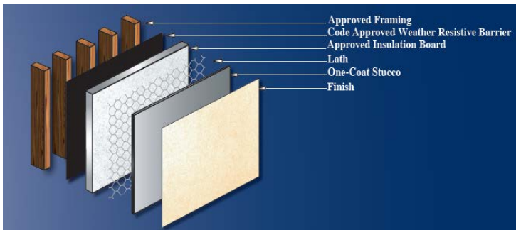
Figure 2: Typical one-coat stucco assembly detail.
