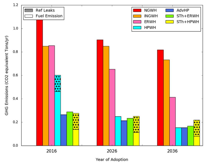
Fig. 2. Average Annual Emissions from source fuel and refrigerant leakage in three adoption years. Efficiencies and refrigerant GWPs improve with time as per schedule given in Table 2.
