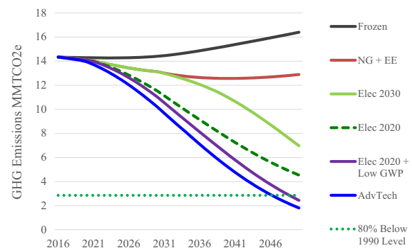
Fig. 7. GHG Emissions trajectories for each Scenario.
