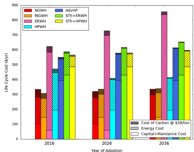
Fig. 3. LCC of WH Technologies in three adoption years. Efficiencies and refrigerant GWPs improve with each adoption year as in Fig. 2.
