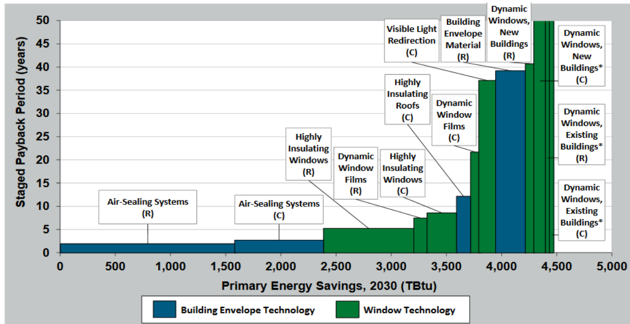
Figure 3 Building Envelope and Window Technology Payback
