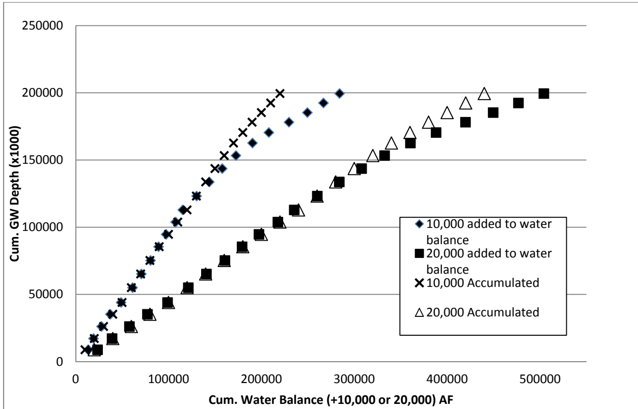
Figure 1 - Comparison between DMC plots when 10,000 AF and 20,000 AF is added to the net water balance
