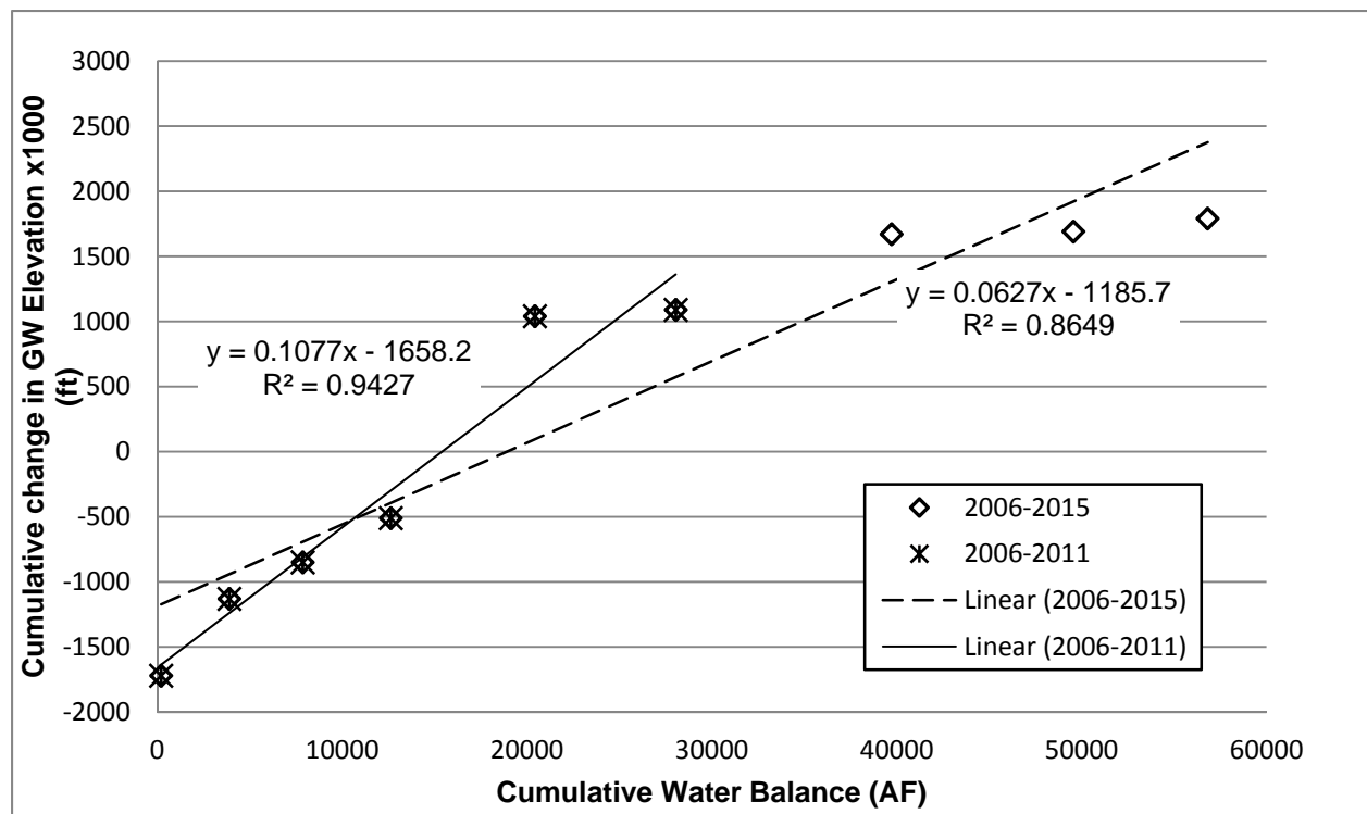
Figure 4 - DMC plot for winter groundwater elevation changes beyond 2006, with a linear regression fit for data points between 2006 and 2011
