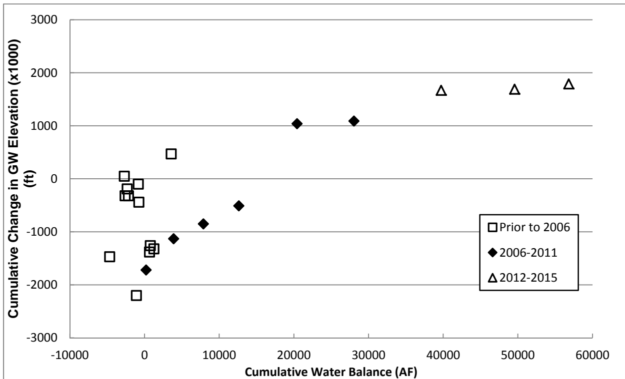
Figure 2 - DMC plot using winter groundwater elevations and net water balance
