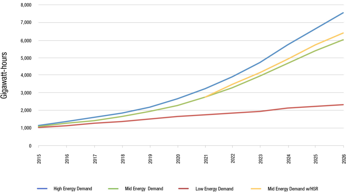
Figure 28: Forecasted Transportation Electricity Demand
