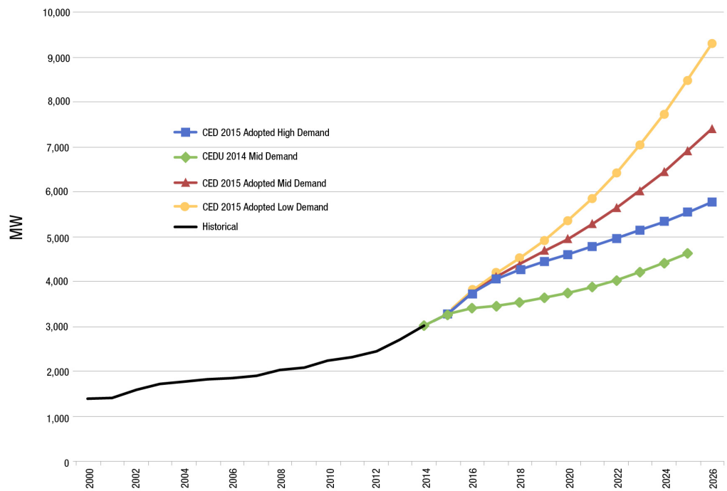
Figure 38: Statewide Self-Generation Peak Reduction Impact
