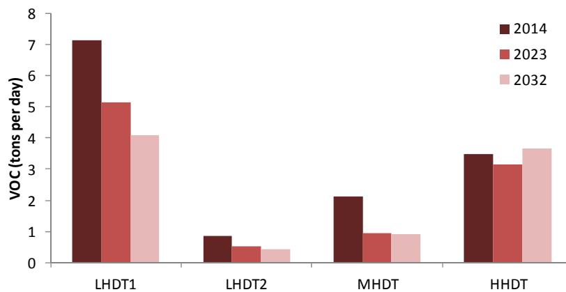
Figure 6. VOC Emissions for Specific On-Road Heavy-Duty Vehicles*
