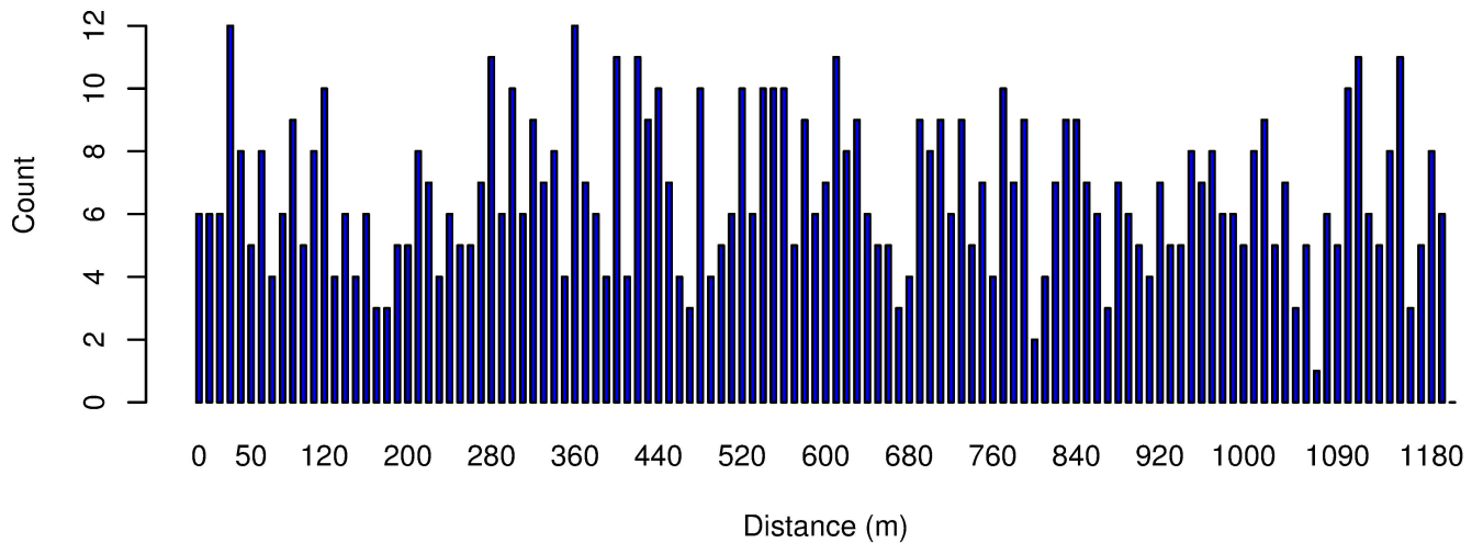
Uniform Distribution
