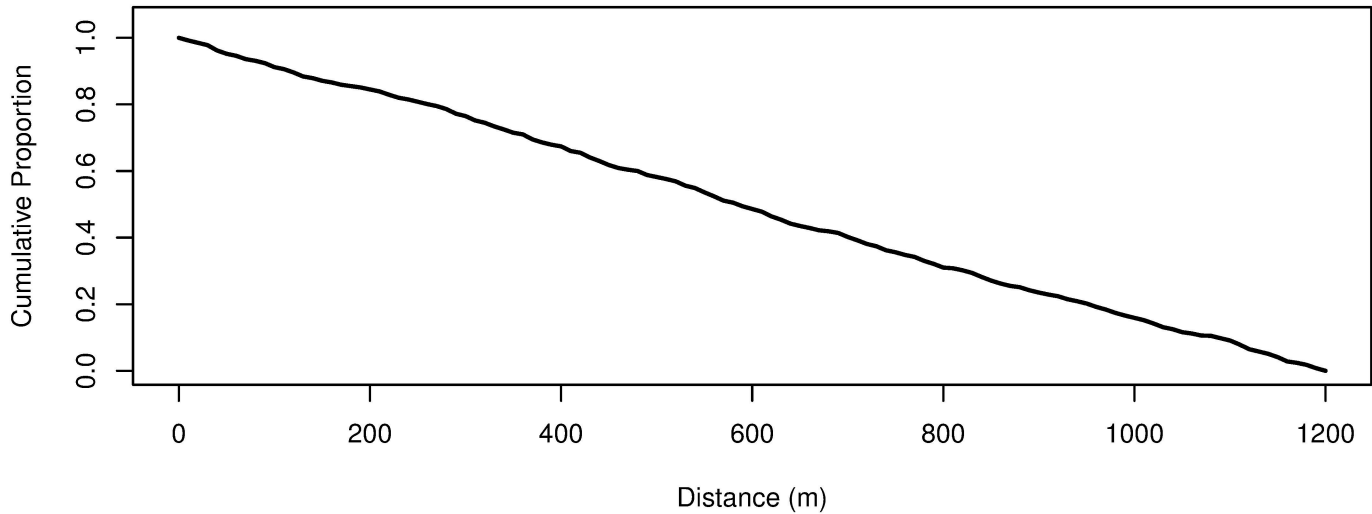
Cumulative Distribution – UNIFORM
