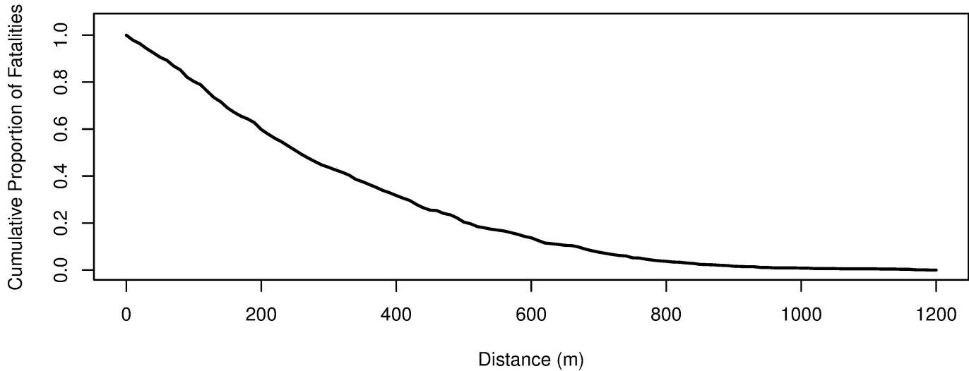
Cumulative Distribution – Half Normal
