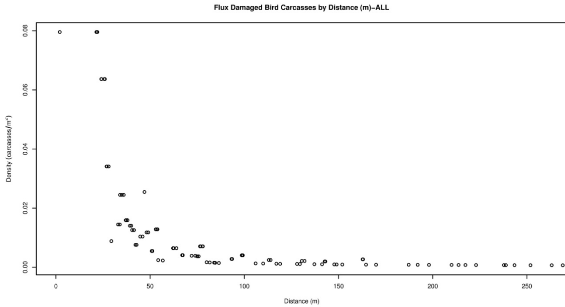
Exhibit 1162. Flux-related carcass density as a function of distance from towers at ISEGS.
