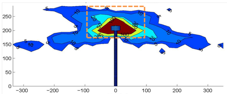
Exhibit 1160. Flux projections for Palen towers, assuming 20% standby, and approximate risk-geometry used to calculate avian exposure to potentially harmful flux.
